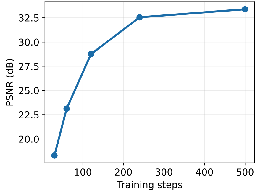
Step sweep: convergence, then plateau near 500 steps
