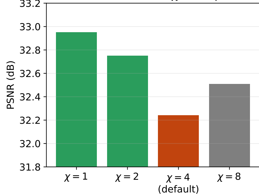
MPS bond-dim sweep: non-monotonic, \chi = 4 dips
