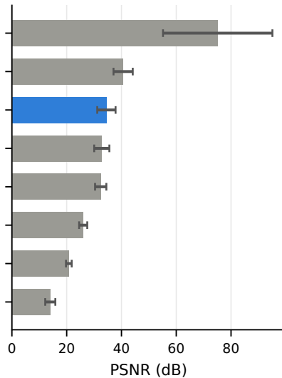
Memorization diagnostic
