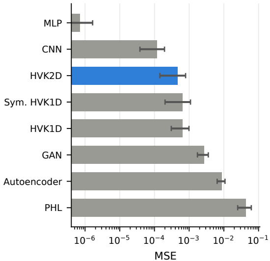
Same-set CIFAR-10
