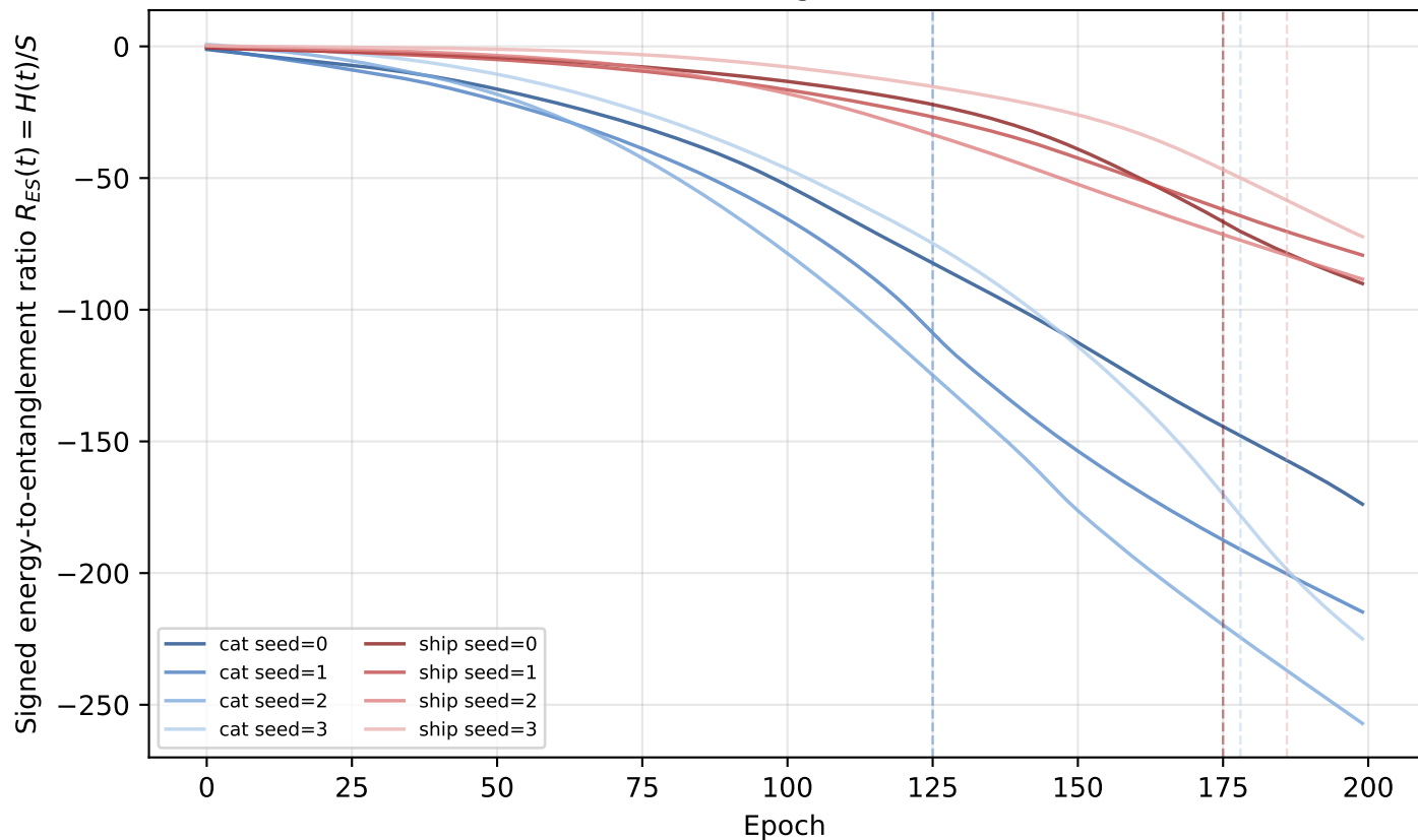
Energy-to-entanglement ratio vs epoch, HVK1D two CIFAR-10 images x four seeds
