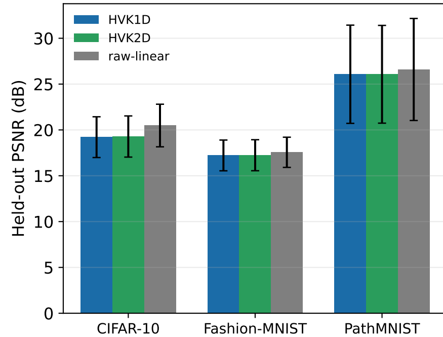
Surrogate sweep (5 seeds): reconstruction
