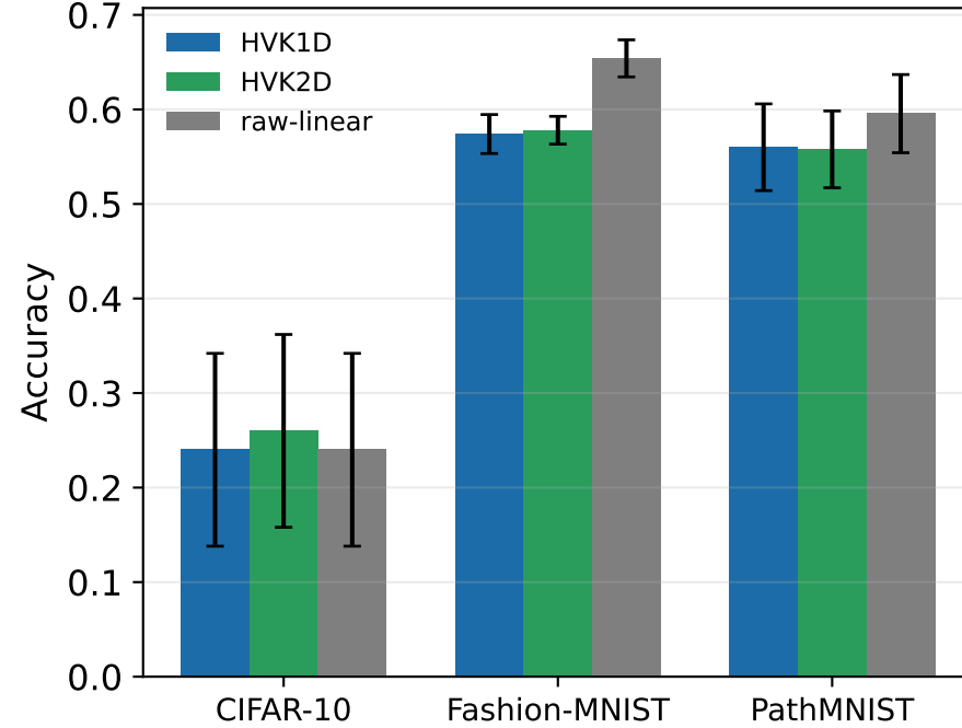
Surrogate sweep (5 seeds): classification
