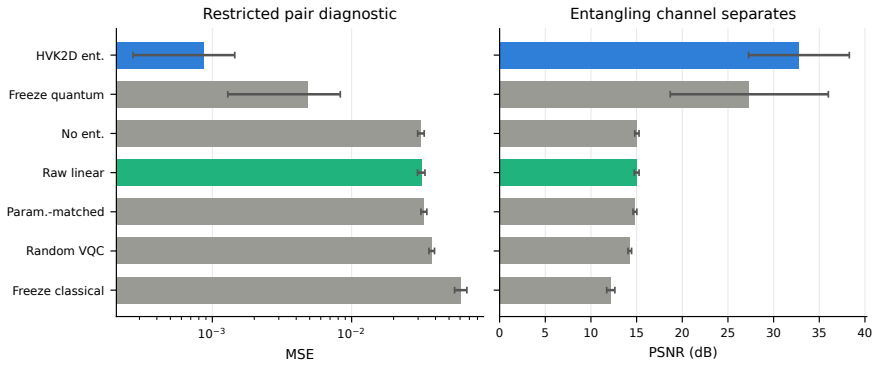
Fig. 6 Restricted pair-correlation diagnostic summary (mean \pm std over five seeds). The entangling observable feature map dominates every control on this deliberately favorable task.
