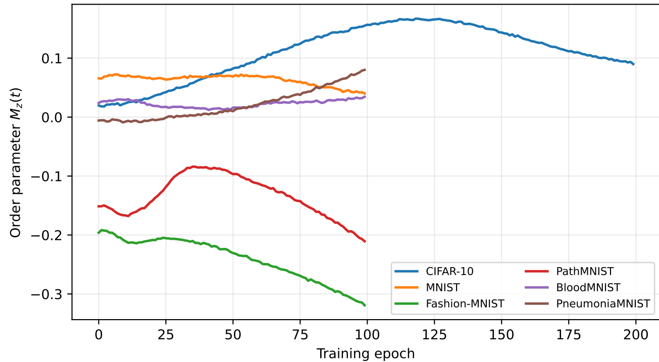
Order-parameter trajectories across datasets (one representative image each)
