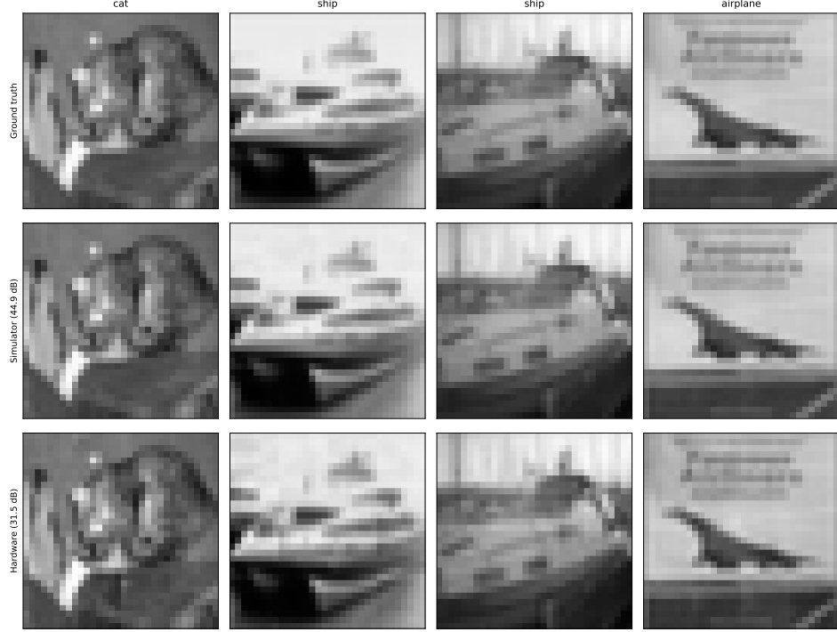
Fig. 3 Four CIFAR-10 images reconstructed from real IBM Quantum hardware measurements (bottom row) against noiseless-simulator replays of the same trained HVK2D checkpoints (middle row) and ground truth (top row).
