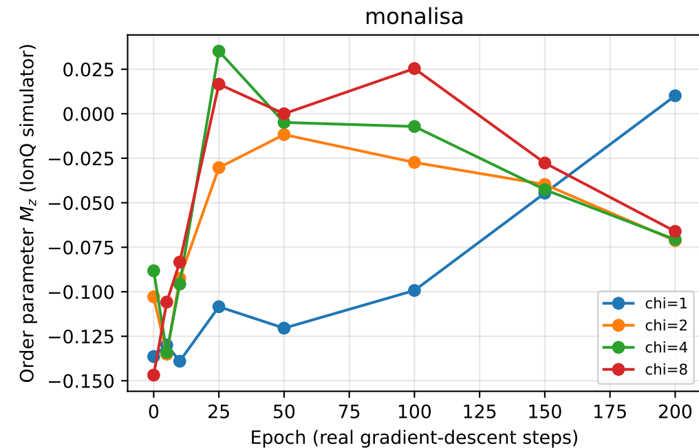
Order parameter vs epoch across MPS bond dimension, real trained checkpoints on ionq_simulator (1024 shots)
