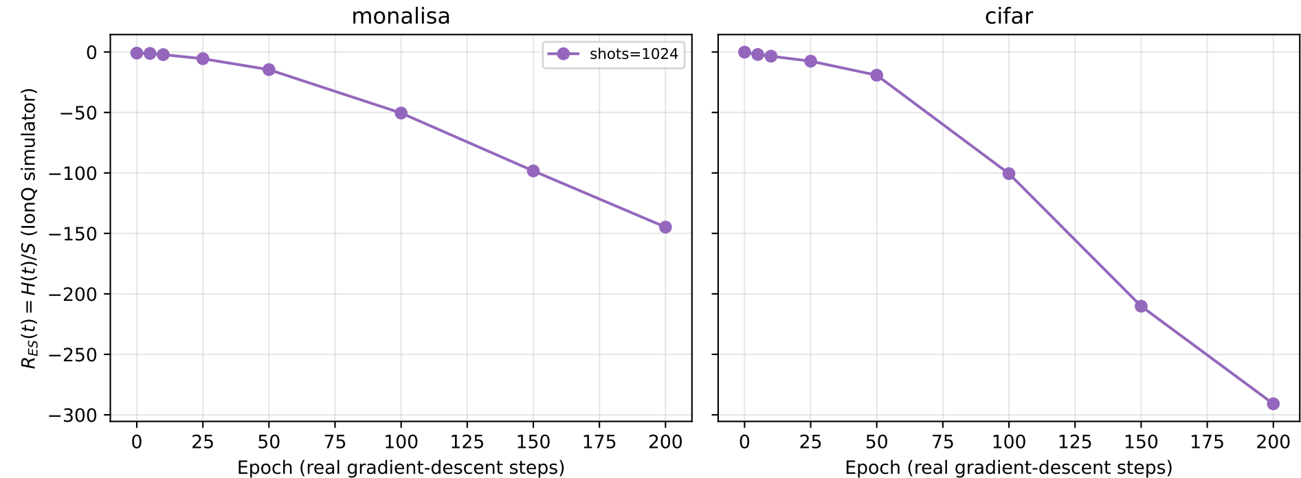
Energy-to-entanglement ratio vs epoch, real trained checkpoints on ionq_simulator
