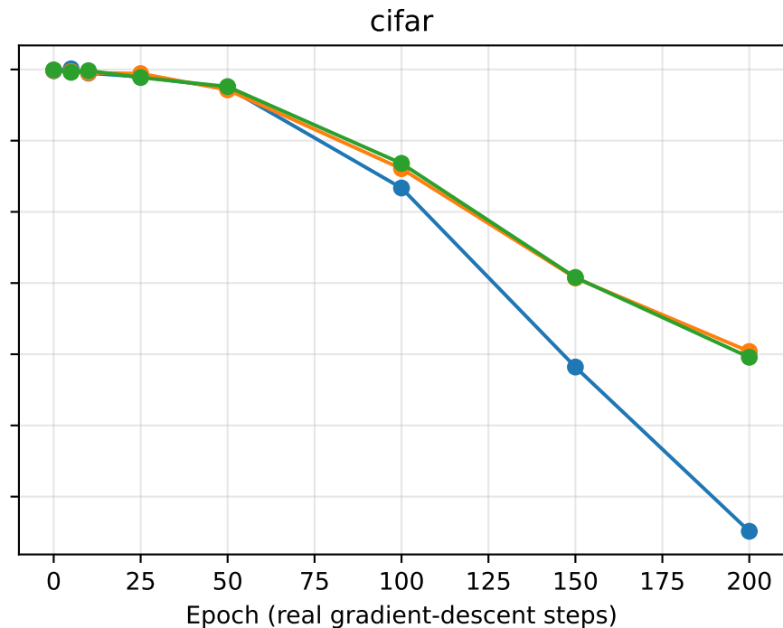
R_ES vs epoch across MPS bond dimension, real trained checkpoints on ibm_marrakesh (1024 shots)
