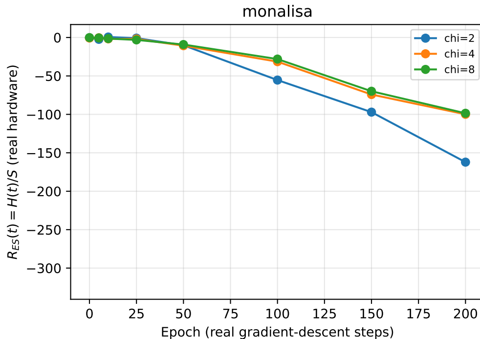
R_ES vs epoch across MPS bond dimension, real trained checkpoints on ibm_marrakesh (1024 shots)
