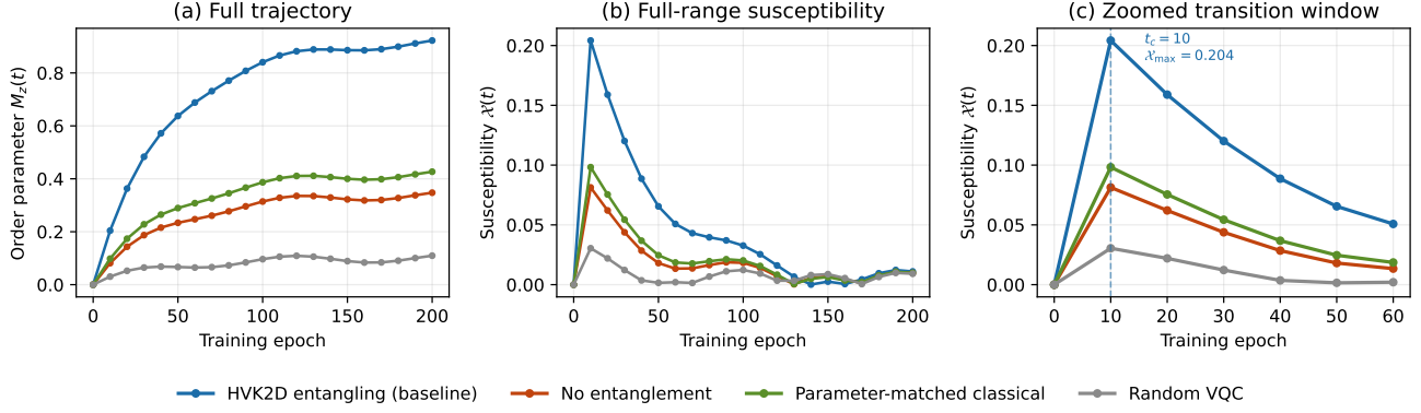
Fig. 7. Order-parameter phase-transition diagnostic on the restricted pair-correlation task. (a) Full order-parameter trajectory M_z(t) and (b) full-range susceptibility \chi(t) ; (c) zooms into the epoch-0–60 transition window, where the entangling channel’s susceptibility peak separates cleanly from every classical control.
