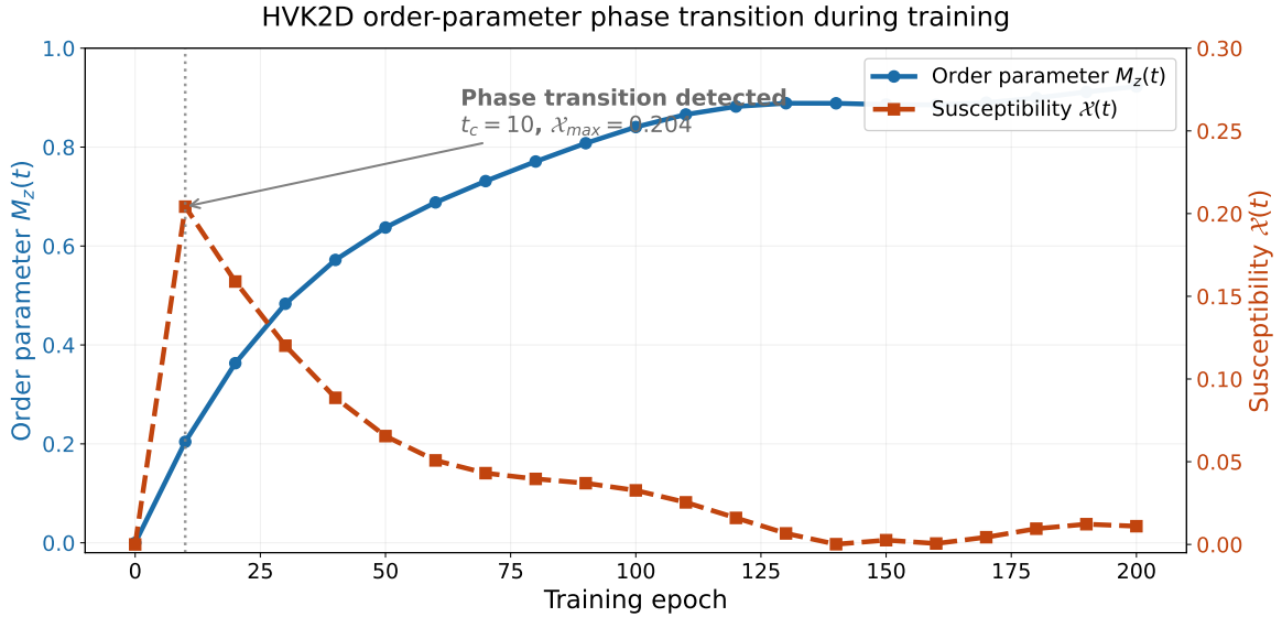
Fig. 6. Order-parameter phase transition for the HVK2D entangling baseline, plotted on a single shared training-epoch axis (x-axis) so the reorganization is visible without cross-referencing separate panels. The solid blue curve (left y-axis) is the order parameter M_z(t) , which rises from 0 toward a plateau near 0.9 as training proceeds. The dashed red curve (right y-axis) is the susceptibility \mathcal{X}(t) = |M_z(t) - M_z(t - \Delta t)| , the epoch-to-epoch rate of change of M_z(t) ; it spikes sharply within the first few epochs and decays smoothly afterward. The vertical dotted gray line and annotated arrow mark the detected critical epoch t_c = 10 , where the susceptibility reaches its maximum value \mathcal{X}_{\max} = 0.204 — the point of most abrupt reorganization in the learned observable field, per the definitions of M_z(t) and \mathcal{X}(t) in Eqs. (??)–(??).
