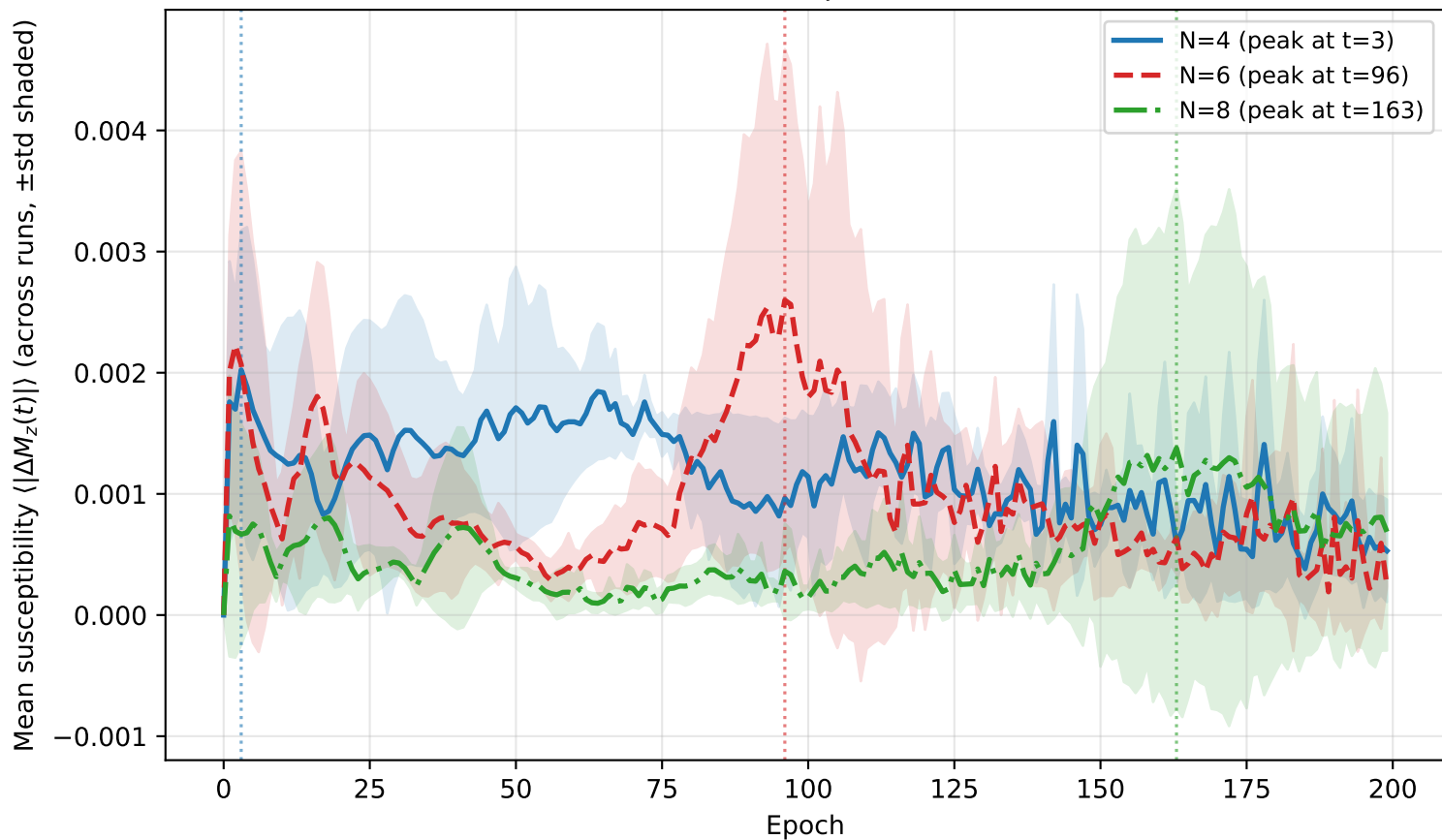
Order-parameter change magnitude vs epoch, qubit-count sweep ensemble mean across 4 runs per N (2 datasets x 2 seeds)
