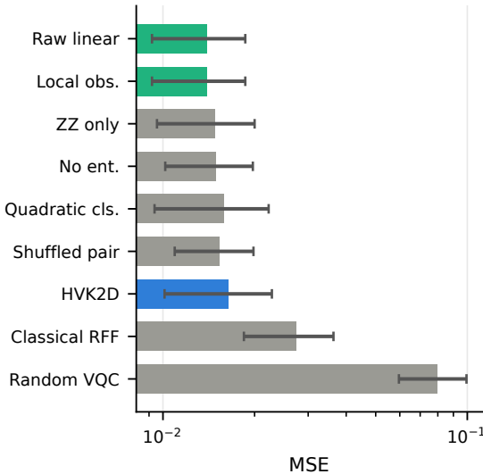
Held-out CIFAR controls
