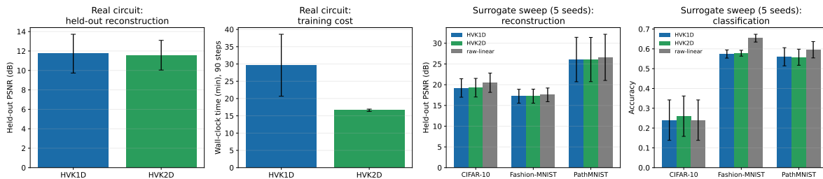
Figure 6: HVK1D vs. HVK2D across both evidence bases. Left two panels: real-circuit held-out PSNR and per-run wall-clock time (90-step budget, 3 seeds, error bars = std). Right two panels: surrogate-sweep held-out reconstruction PSNR and classification accuracy across three datasets (5 seeds), both topologies plotted against the strongest classical control (raw-linear).
