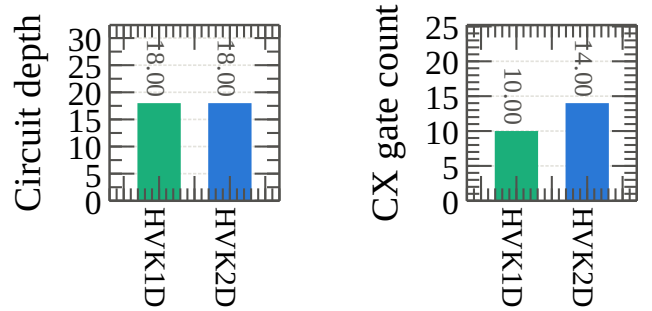
Fig. 8. IBM Cloud circuit-resource summary for the HVK1D and HVK2D hardware probes.
