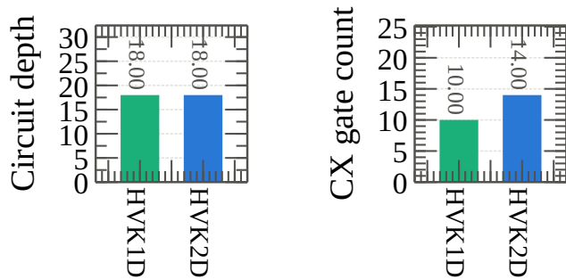
Fig. 8. IBM Cloud circuit-resource summary for the HVK1D and HVK2D hardware probes.
