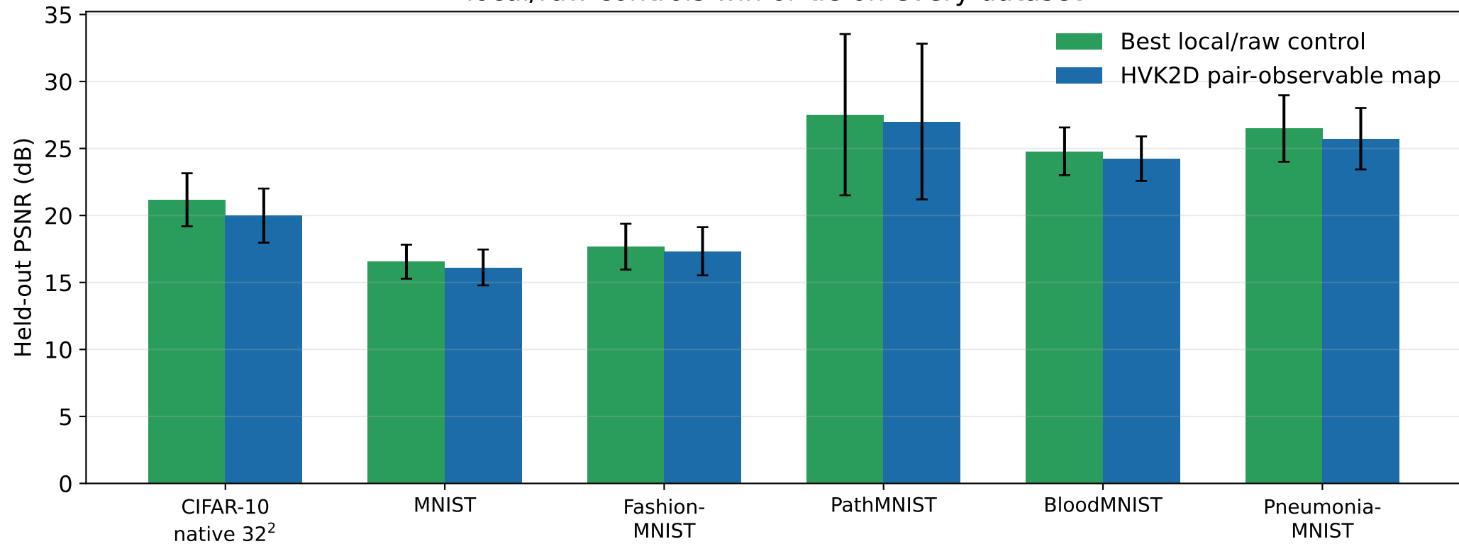
Held-out reconstruction across six real datasets: local/raw controls win or tie on every dataset
