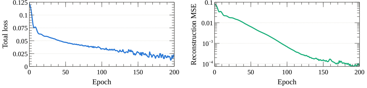
Figure 5: Training dynamics for the contrastive Hamiltonian-core run of Table 11: total loss (left) and reconstruction MSE on a log scale (right) over 200 epochs. Both converge smoothly with no instability introduced by the contrastive energy term.
