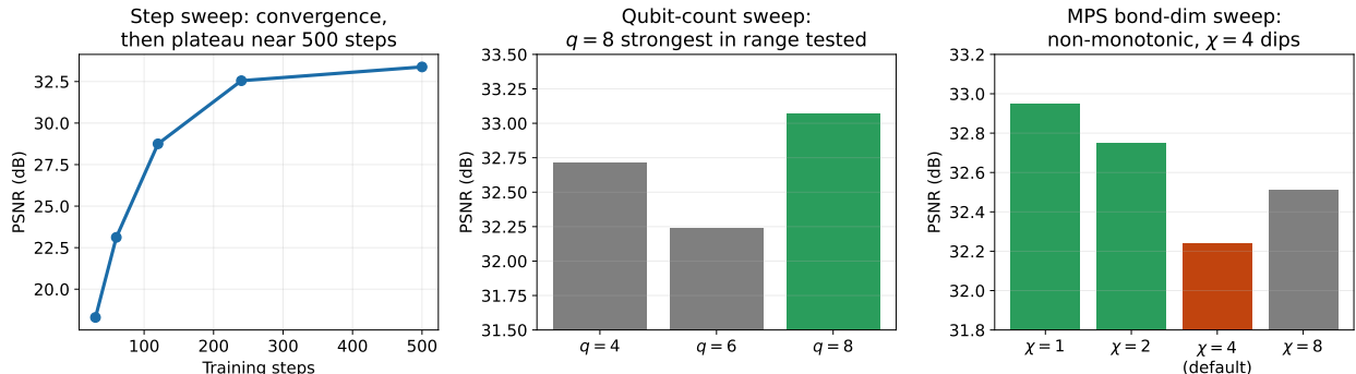
Figure 3: Capacity and scaling sweeps from Table 8 (single-seed, Monalisa ). Left: PSNR vs. training steps, confirming convergence-limited behavior with a plateau near 500 steps. Center: qubit-count sweep, q = 8 strongest in the tested range. Right: MPS bond-dimension sweep, highlighting the non-monotonic dip at the default \chi = 4 (orange) relative to both smaller ( \chi = 1, 2 , green) and larger ( \chi = 8 , gray) bond dimensions.
