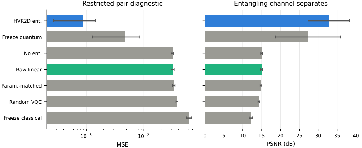
Figure 7: The restricted pair-correlation diagnostic underlying the entanglement-necessity result (mean R^2 = 0.9735 vs. R^2 \leq 0.02 for non-entangling controls), shown here as MSE (left) and PSNR (right) across the full variant set: the trained HVK2D entangling map, freeze-quantum, no-entanglement, raw-linear, parameter-matched classical, random-VQC, and freeze-classical. The entangling channel (blue) separates numerically from every non-entangling control on this target, in direct contrast to the ordinary held-out reconstruction result of Section 3.2 where the same entangling channel does not separate from local/raw controls — the two figures together visualize this document’s central task-dependence argument.
