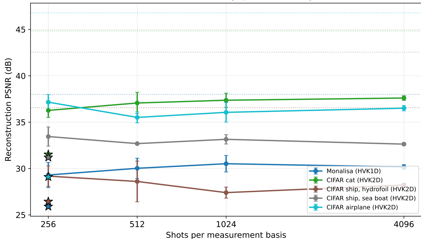
Noise/shot trade-off: ideal (dotted) vs. FakeFez-noisy simulation (lines) vs. real IBM hardware (★, at 256 shots)
