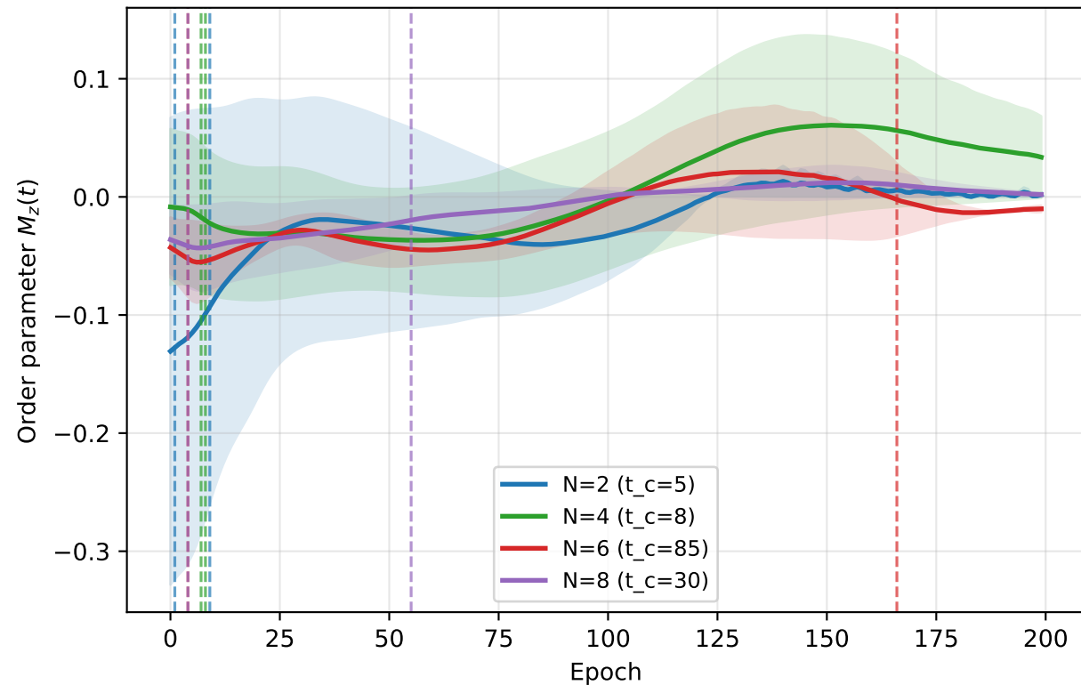
Order parameter vs epoch across N, monalisa (mean +/- std over seeds; dashed = detected critical epoch)
