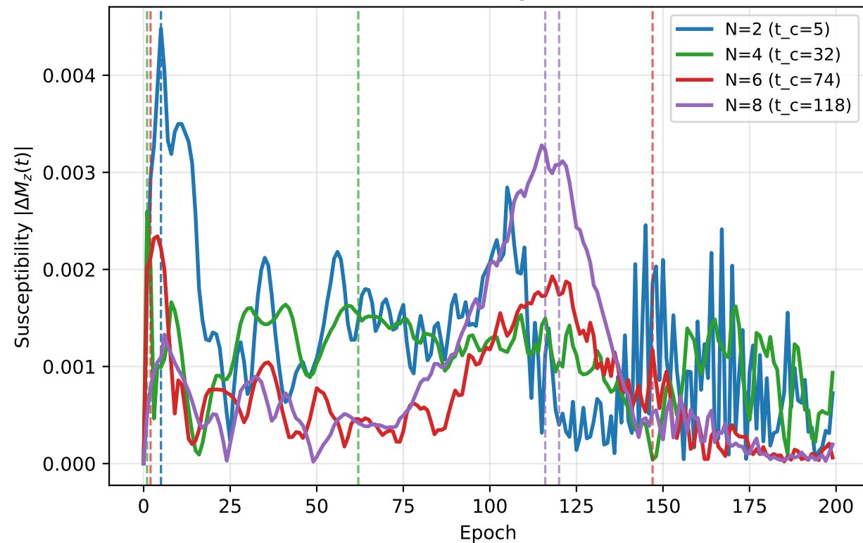
Phase transition signal across N
