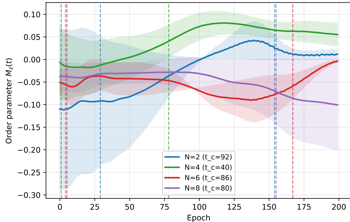
Order parameter vs epoch across N, 0002_ship_sea_boat_s_001456 (mean +/- std over seeds; dashed = detected critical epoch)
