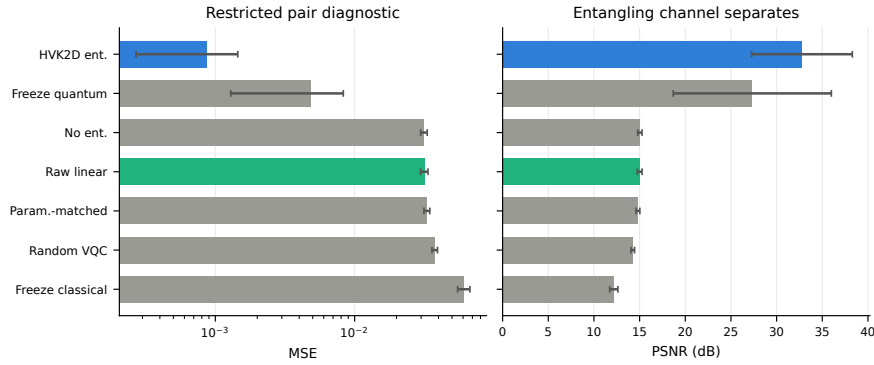
Fig. 6 Restricted pair-correlation diagnostic summary (mean \pm std over five seeds). The entangling observable pair-observable feature map dominates every control on this deliberately favourable task.
