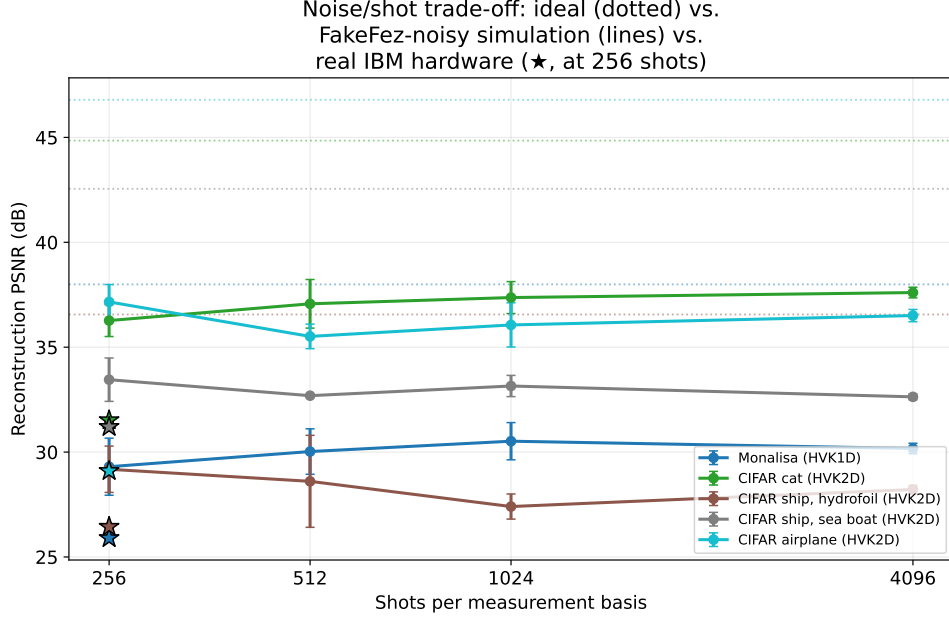
Fig. 4 Calibrated device-noise simulation ( FakeFez , mean \pm std over three executions). Dotted lines show noiseless ceilings and stars show real-hardware measurements. Increasing 256 to 4096 shots changes mean PSNR by only -0.05 dB.
