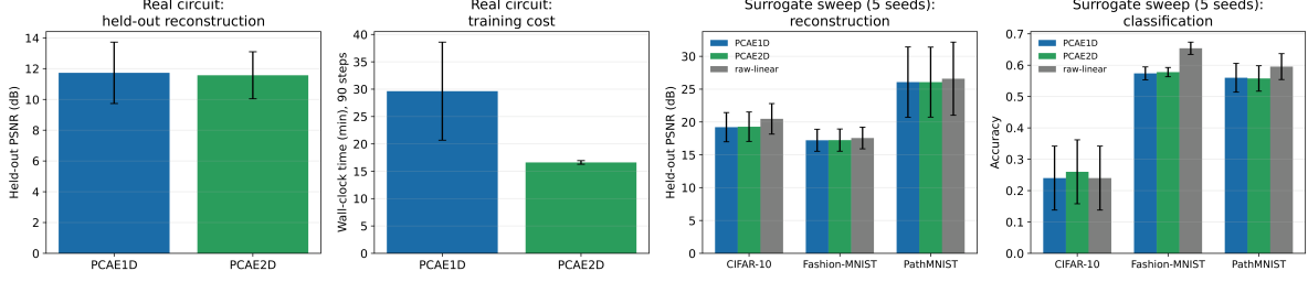
Figure 6: PCAE1D vs. PCAE2D across both evidence bases. Left two panels: real-circuit held-out PSNR and per-run wall-clock time (90-step budget, 3 seeds, error bars = std). Right two panels: surrogate-sweep held-out reconstruction PSNR and classification accuracy across three datasets (5 seeds), both topologies plotted against the strongest classical control (raw-linear).
