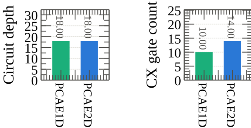
Figure 8: Transpiled circuit resource comparison between the PCAE1D ( Monalisa ) and PCAE2D (CIFAR) per-patch circuits at optimization_level=1 on ibm_fez : circuit depth (left) and CX-gate count (right). Both circuits have depth 18 and use 10–14 CX gates. These resource counts document the executed circuits; they do not by themselves attribute the observed hardware–simulator PSNR gap to a particular noise source.
