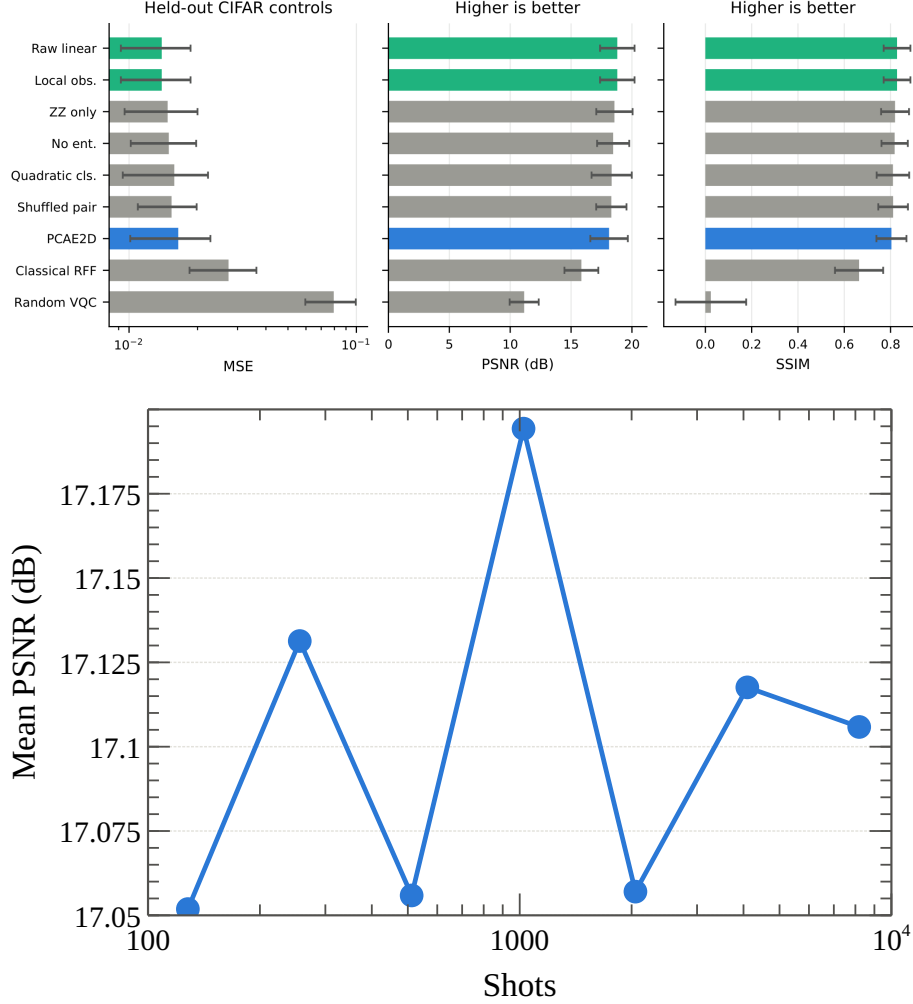
Figure 1: Held-out CIFAR-10 reconstruction and shot-noise robustness. The raw/local comparison passes TOST before, but not after, Holm correction; PCAE2D exceeds the random-VQC null control.
