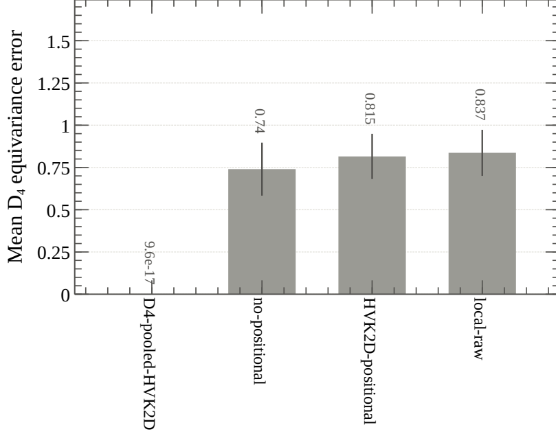
Fig. 5 D_4 equivariance diagnostic. The unpooled positional map is not equivariant; the group-pooled map is equivariant to numerical precision. The group-pooled map is equivariant to numerical precision. The unpooled positional map is not.
