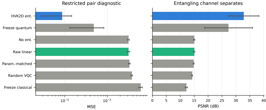
Fig. 6 Restricted pair-correlation diagnostic summary (mean \pm std over five seeds). The entangling observable pair-observable feature map dominates every control on this deliberately favourable task.
