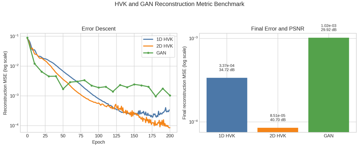
Figure 5: Reconstruction metric comparison for 1D HVK, 2D HVK, and the GAN baseline on the Monalisa image reconstruction task. The left panel shows MSE descent over training on a logarithmic scale. The right panel compares final MSE and the corresponding PSNR. Lower MSE and higher PSNR indicate better reconstruction quality.
