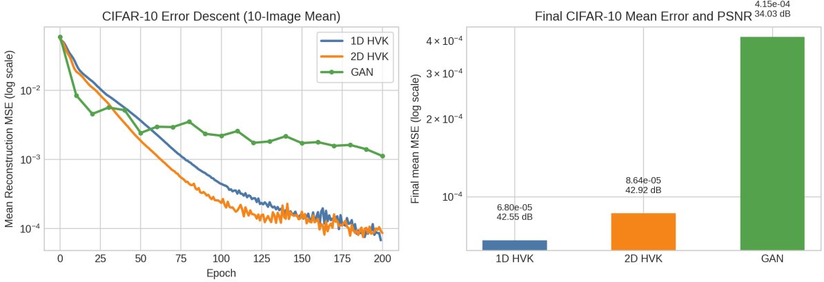
Figure 6: CIFAR-10 test subset reconstruction metric comparison for 1D HVK, 2D HVK, and the GAN baseline. The left panel shows average MSE descent over 200 training epochs. The right panel compares the average final MSE and the corresponding PSNR across the 10-image test subset.
