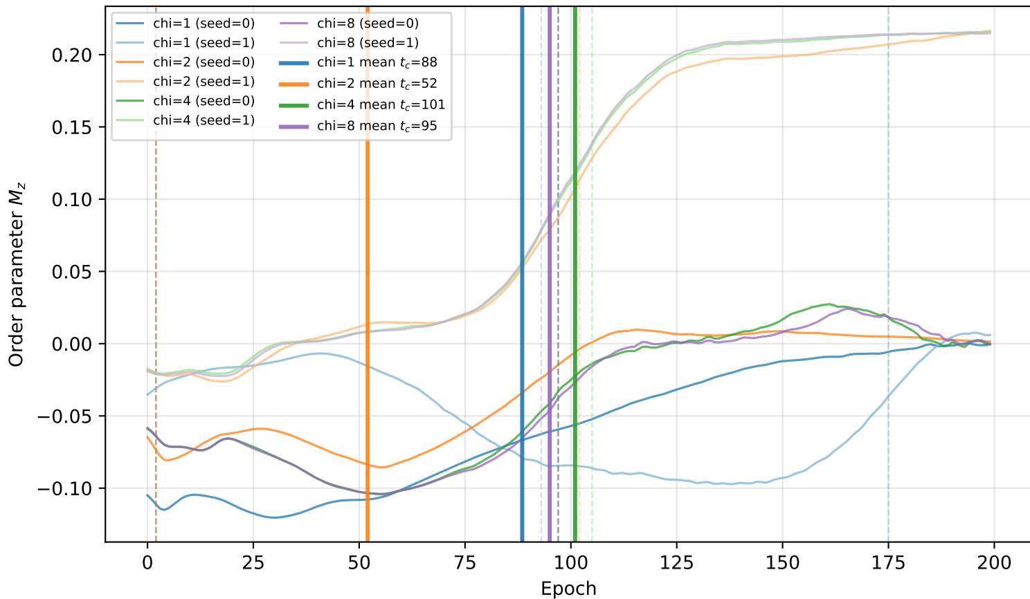
MPS bond-dimension comparison: order parameter vs epoch (N=6 fixed) dashed lines mark each run's detected critical epoch
