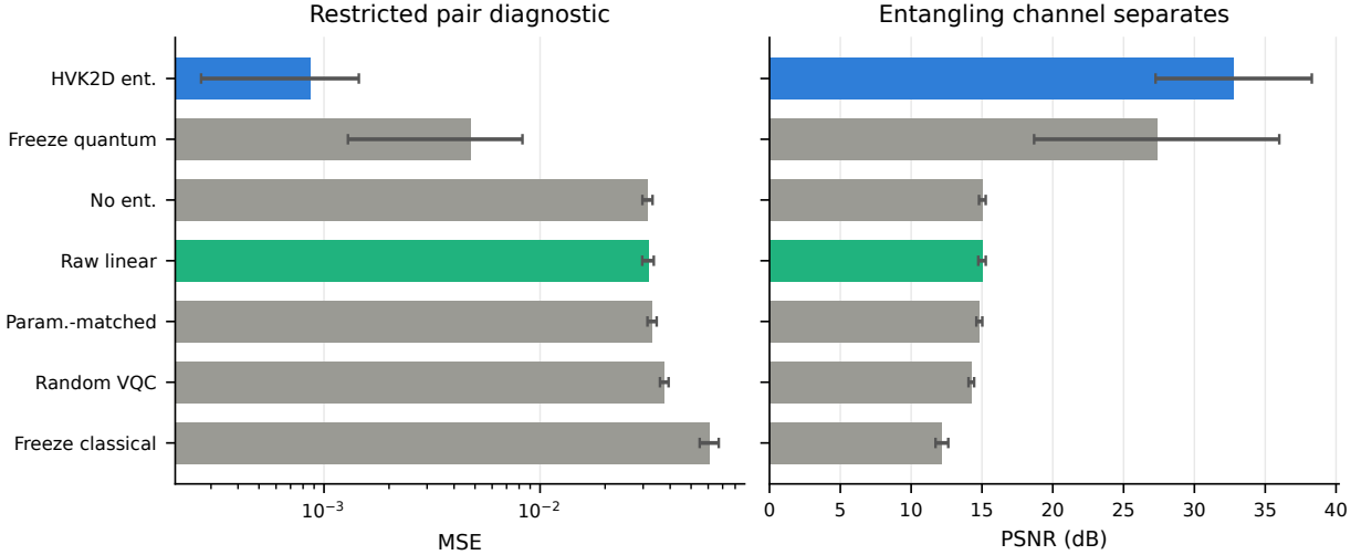
Figure 4: The restricted pair-correlation diagnostic underlying the entanglement-necessity result (mean R^2 = 0.9735 vs. R^2 \leq 0.02 for non-entangling controls), shown here as MSE (left) and PSNR (right) across the full variant set: the trained HVK2D entangling map, freeze-quantum, no-entanglement, raw-linear, parameter-matched classical, random-VQC, and freeze-classical. The entangling channel (blue) separates numerically from every non-entangling control on this target, in direct contrast to the ordinary held-out reconstruction result of Section 3.3 where the same entangling channel does not separate from local/raw controls — the two figures together visualize this document’s central task-dependence argument.
