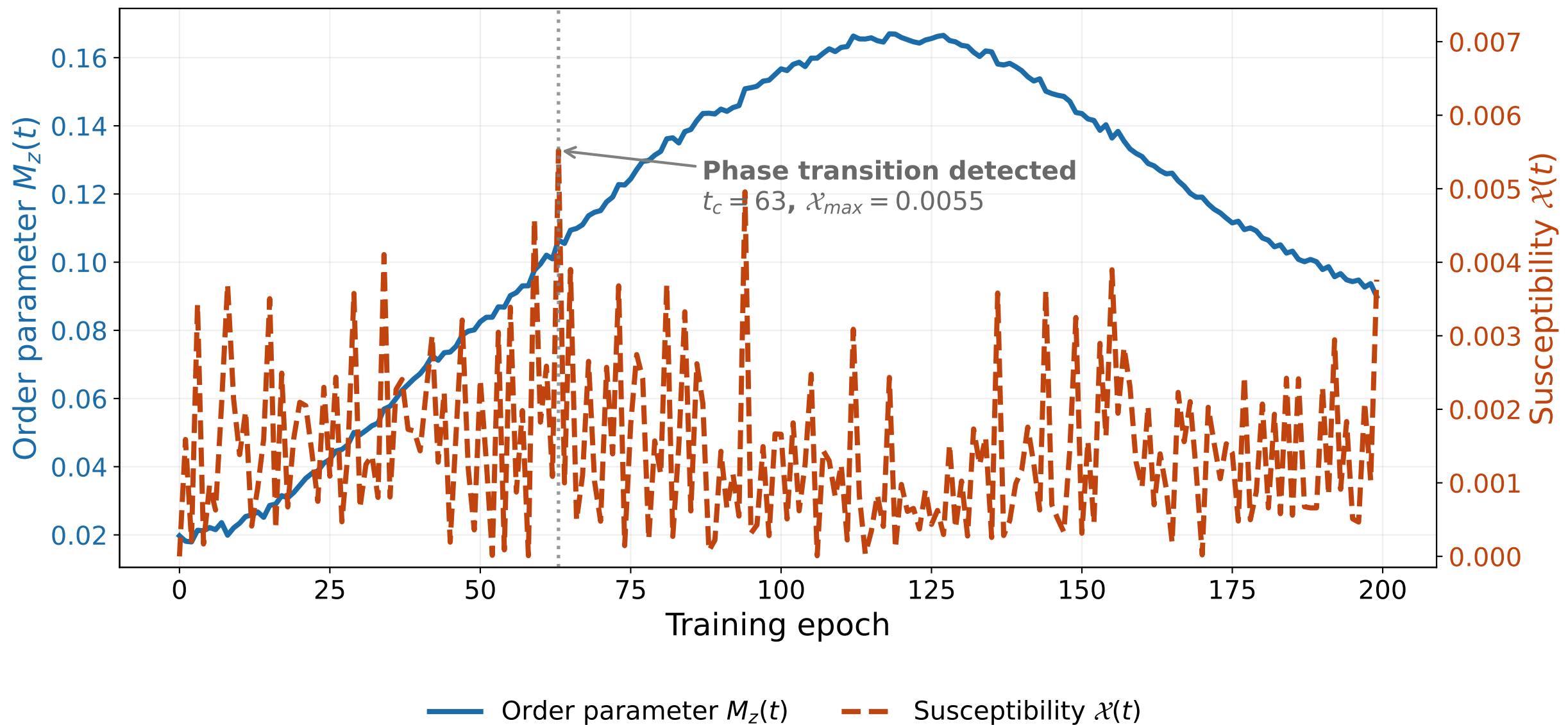
Order-parameter phase transition: CIFAR-10 "cat" image reconstruction (HVK2D)
