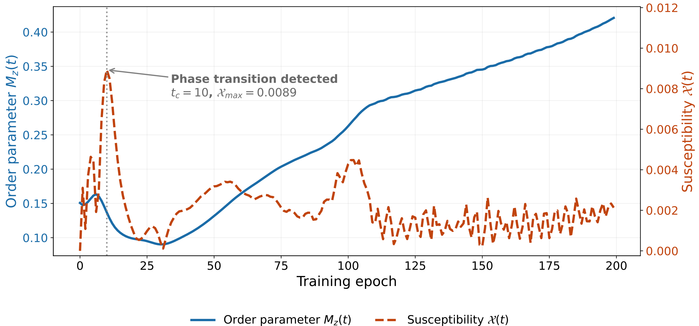
Order-parameter phase transition: MonaLisa reconstruction (HVK1D)
