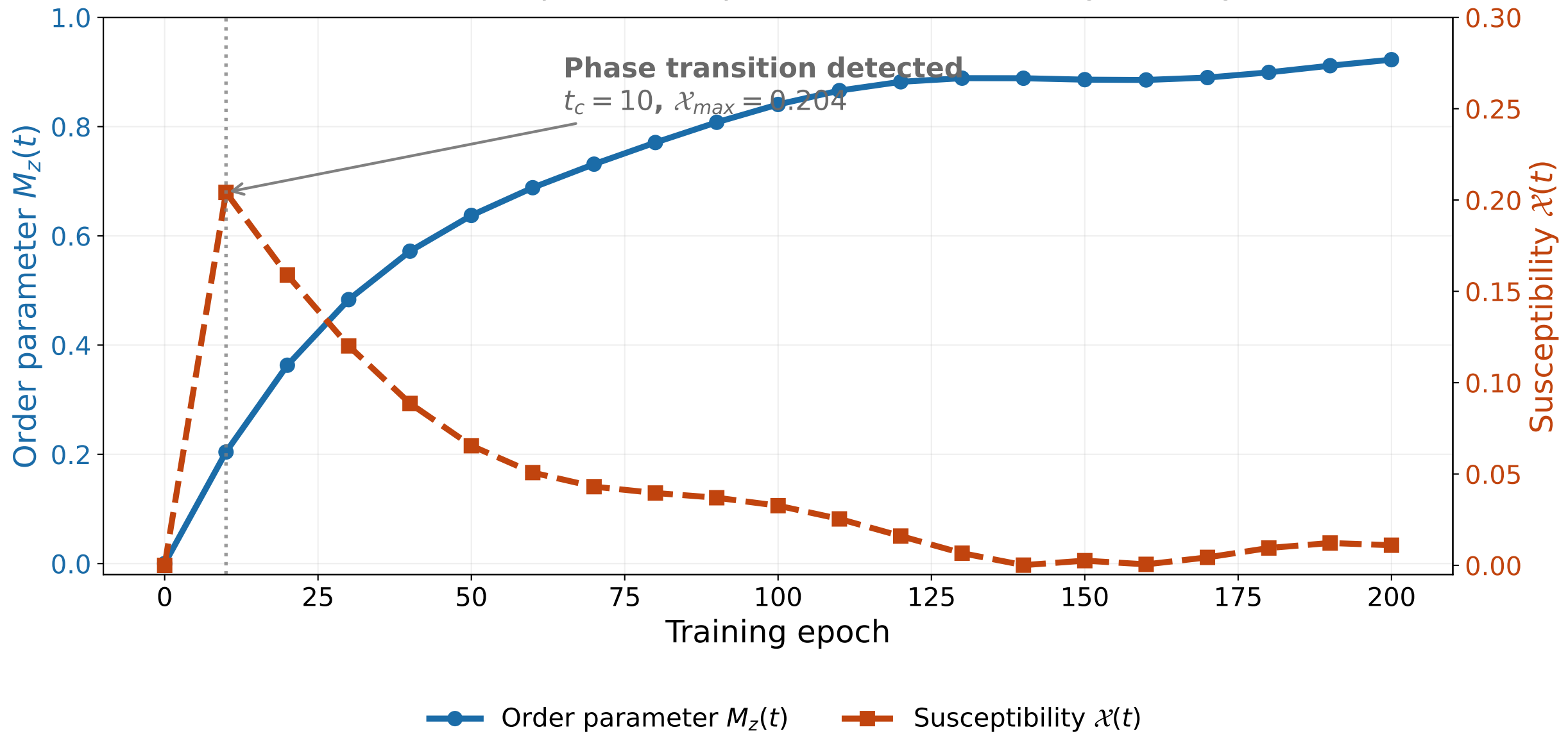
HVK2D order-parameter phase transition during training
