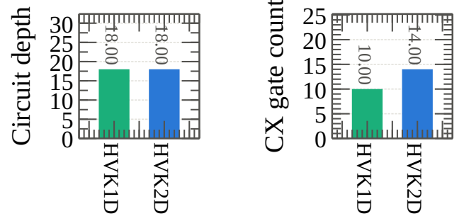
Fig. 6. IBM Cloud circuit-resource summary for the HVK1D and HVK2D hardware probes.
