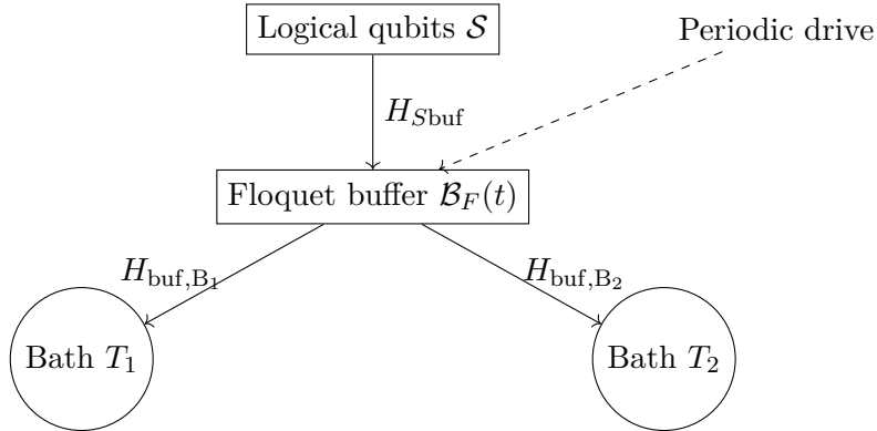
Figure 27: Periodically driven logic gate with Floquet buffer. The logical qubits interact only with the driven buffer; the buffer couples to thermal reservoirs. The device is not fully autonomous: a classical clock synchronises the drive and the stroboscopic readout.
