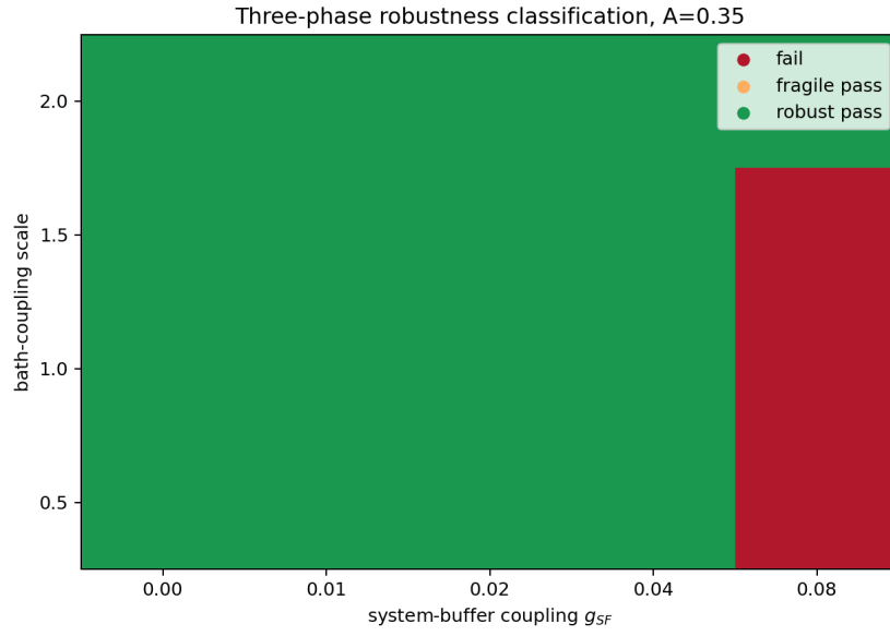
Figure 15: Three–phase classification (robust pass / fragile / fail), analogous to CMOS noise–margin analysis.
