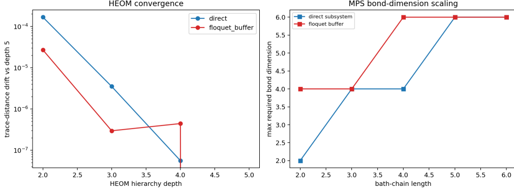
Figure 13: Scaling validation. Left: HEOM convergence versus hierarchy depth, measured by trace-distance drift relative to depth 5. Right: estimated MPS bond dimension versus structured-bath chain length for the direct subsystem and the Floquet-buffered subsystem.
