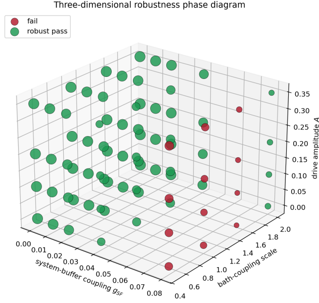
Figure 16: Three-dimensional robustness phase diagram over drive amplitude, bath-coupling scale, and system-buffer coupling; marker size scales with the buffered decoding margin.
