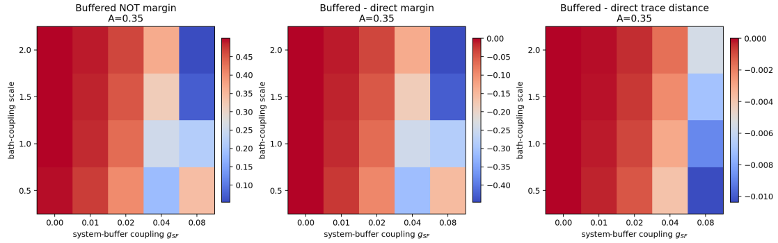
Figure 19: GKSL robustness phase maps at the largest drive amplitude: buffered margin, buffered–direct margin, and trace–distance gain over system–buffer and bath–coupling scales.
