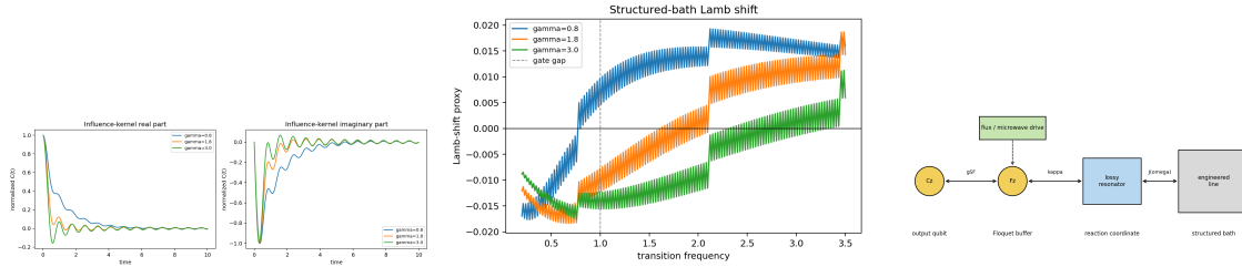
Figure 17: Supporting theory and implementation figures. Left: path-integral influence-memory kernel for different bath cutoffs. Middle: structured-bath Lamb-shift proxy showing drive/bath-induced detuning risk near the gate gap. Right: practical circuit-QED implementation route for the output buffer and engineered reservoir.
