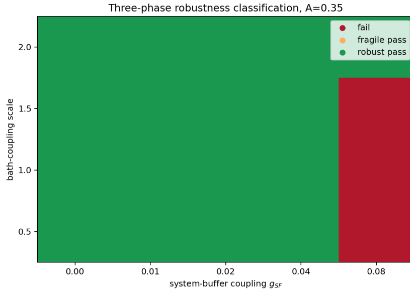
Figure 20: Three–phase classification (robust pass / fragile / fail), analogous to CMOS noise–margin analysis.
