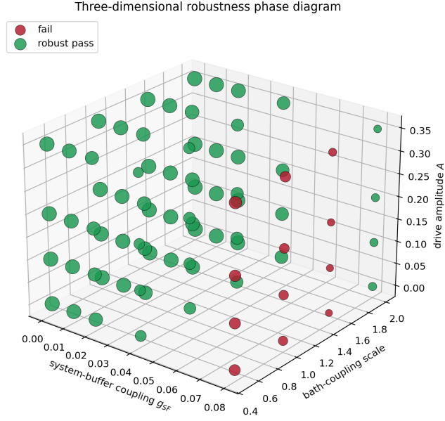
Figure 15: Three-dimensional robustness phase diagram over drive amplitude, bath-coupling scale, and system-buffer coupling; marker size scales with the buffered decoding margin.
