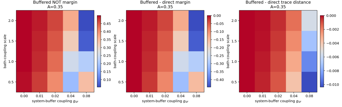
Figure 13: GKSL robustness phase maps at the largest drive amplitude: buffered margin, buffered–direct margin, and trace–distance gain over system–buffer and bath–coupling scales.
