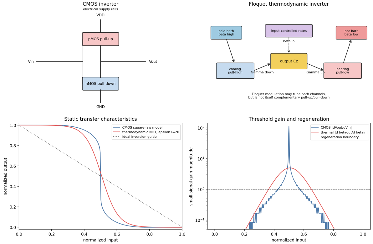
Figure 26: CMOS and thermodynamic-inverter comparison generated from code. Top: complementary electrical pull-up/pull-down and the corresponding cold-rail cooling / hot-rail heating architecture. Bottom: normalized transfer curves and small-signal gain. The thermodynamic NOT has a regenerative G > 1 region, but the present Floquet buffer is a tunable spectral stage rather than a complete complementary inverter.
