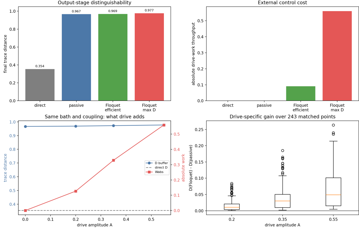
Figure 25: Architecture-level HEOM comparison. Top: distinguishability and external drive throughput for direct, passive, and two driven operating points. Bottom left: adding drive at one fixed bath/coupling point gives a small increase in D while work grows. Bottom right: distribution of the drive-specific increment over all 243 matched driven/passive pairs.
