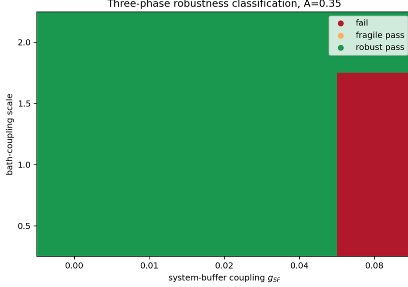
Figure 28: Three-phase classification (robust pass / fragile / fail), analogous to CMOS noise-margin analysis.
