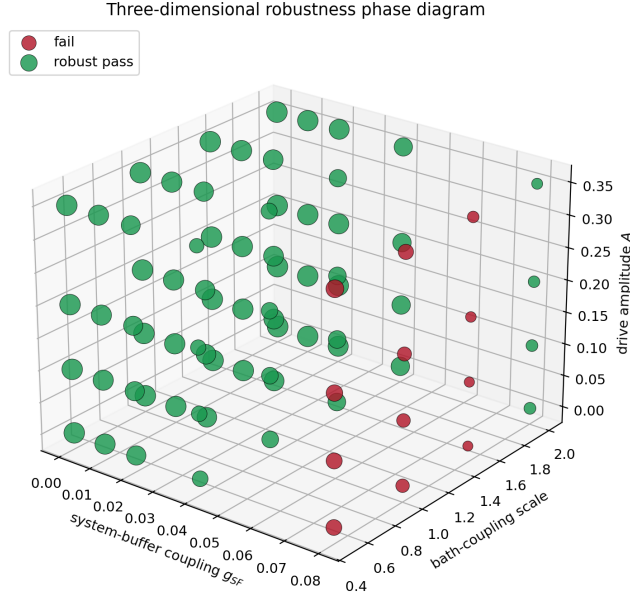
Figure 29: Three-dimensional robustness phase diagram over drive amplitude, bath-coupling scale, and system-buffer coupling; marker size scales with the buffered decoding margin.
