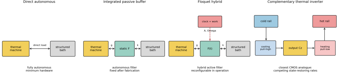
Figure 24: Four architecture classes. Direct contact minimizes hardware; the static integrated buffer preserves autonomy while filtering the bath; the Floquet hybrid adds in-operation spectral control; and a genuinely CMOS-like thermal inverter requires complementary pull-high and pull-low dissipative channels rather than one buffer alone.
