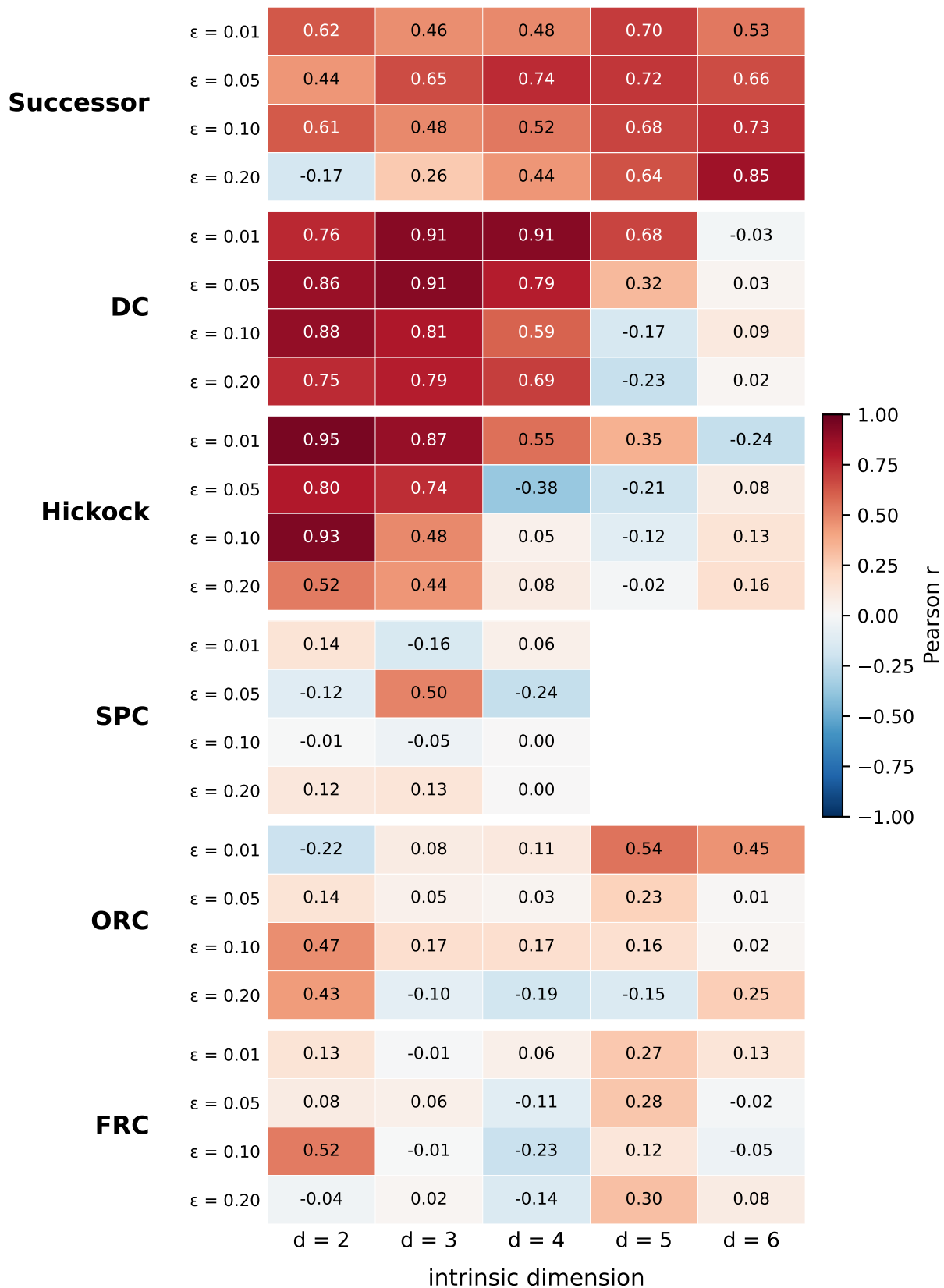
Curvature recovery on the Colosseum benchmark
