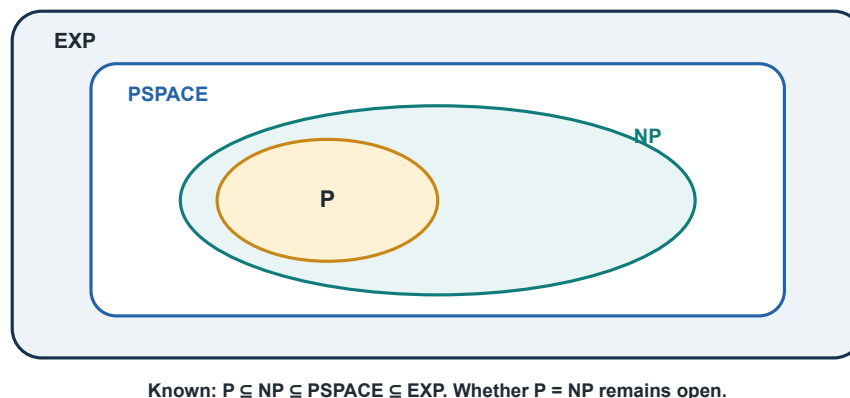
Figure 7.1: Nested regions show P contained in NP, NP contained in PSPACE, and PSPACE contained in EXP; the equality of P and NP remains open.
