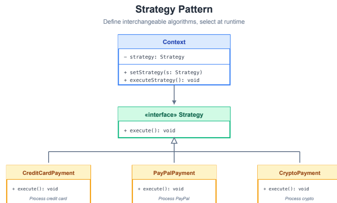
Figure 4.21: Strategy Pattern
