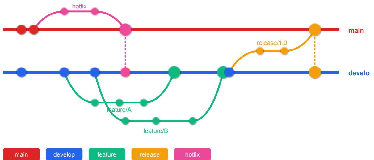
Figure 1.7: Gitflow
