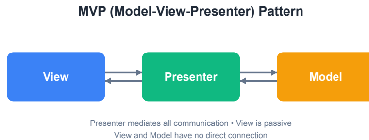
Figure 4.3: MVP (Model-View-Presenter) Pattern
