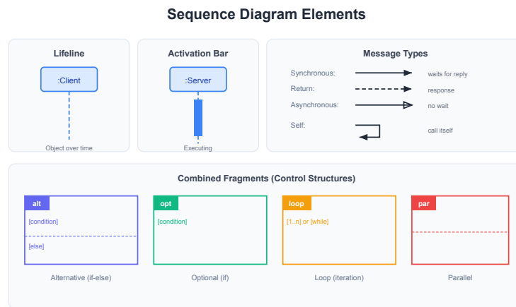
Figure 3.7: UML sequence notation for participants, lifelines, activations, and messages
