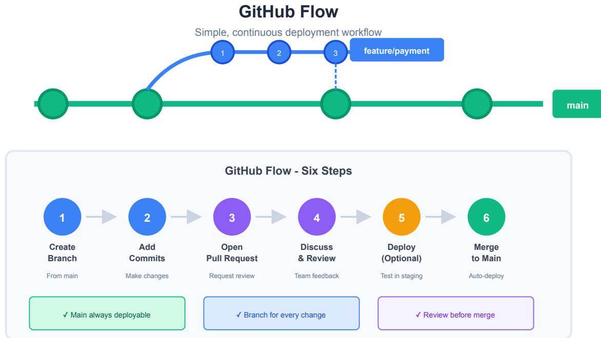
Figure 7.8: GitHub Flow branching strategy
