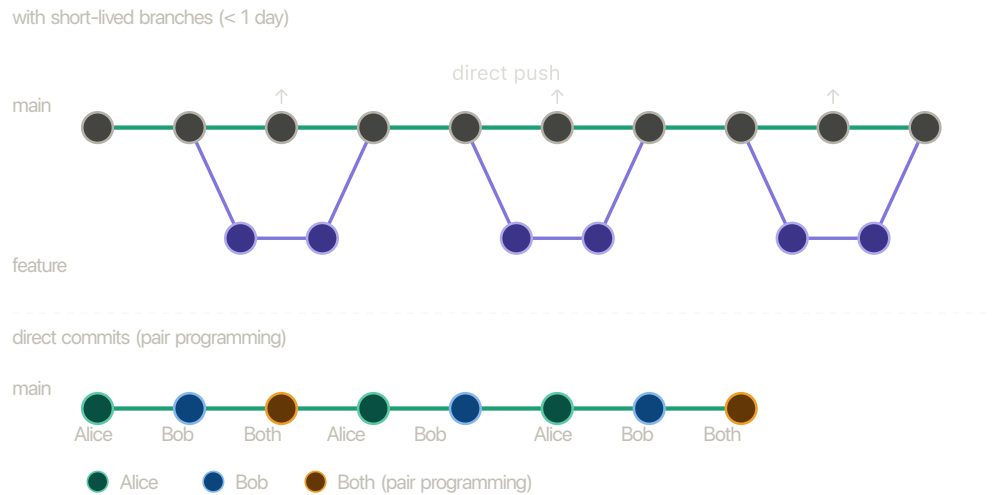
Figure 7.9: Trunk-based development with short-lived branches
