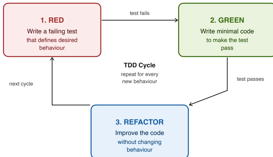
Figure 8.3: Test-driven development cycle: red, green, and refactor
