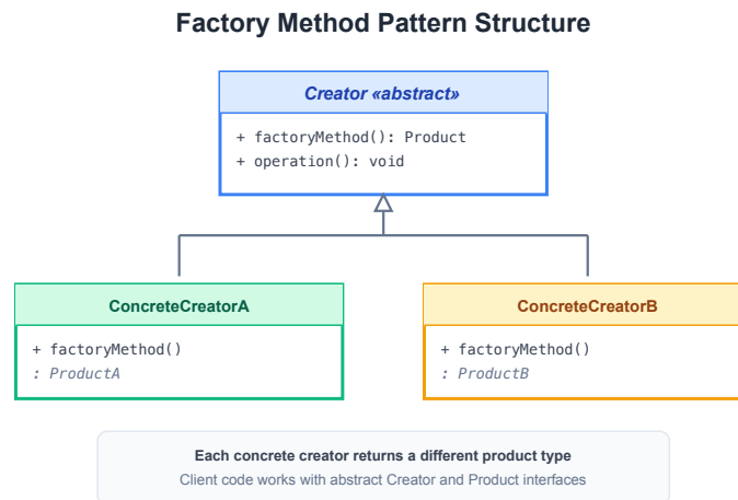
Figure 4.16: Factory Method Pattern Structure
