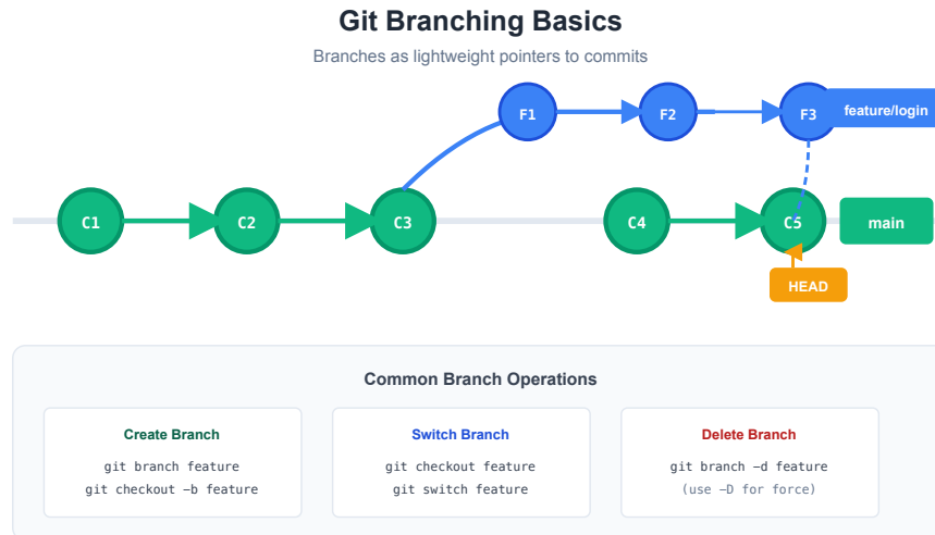
Figure 7.1: Git branching basics - branches as pointers
