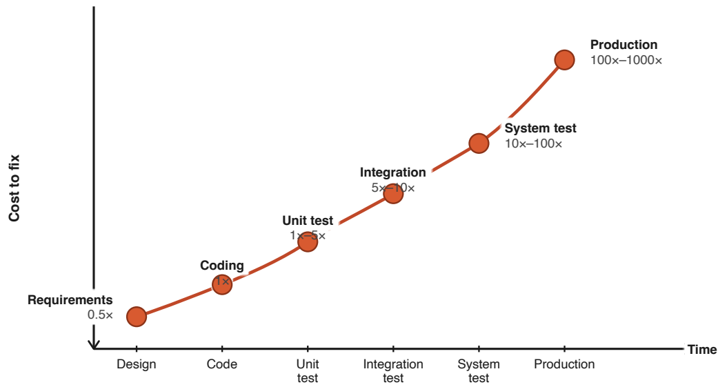
Figure 8.1: Cost to fix defects rising across lifecycle stages
