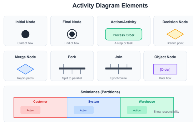
Figure 3.4: UML activity notation for actions, decisions, flow, and initial and final nodes
