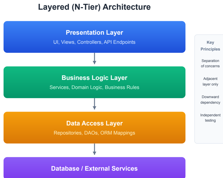
Figure 4.1: Layered Architecture - Four-Tier Configuration
