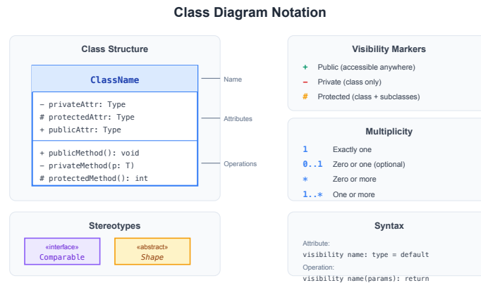
Figure 3.9: UML class notation showing name, attributes, operations, visibility, and types
