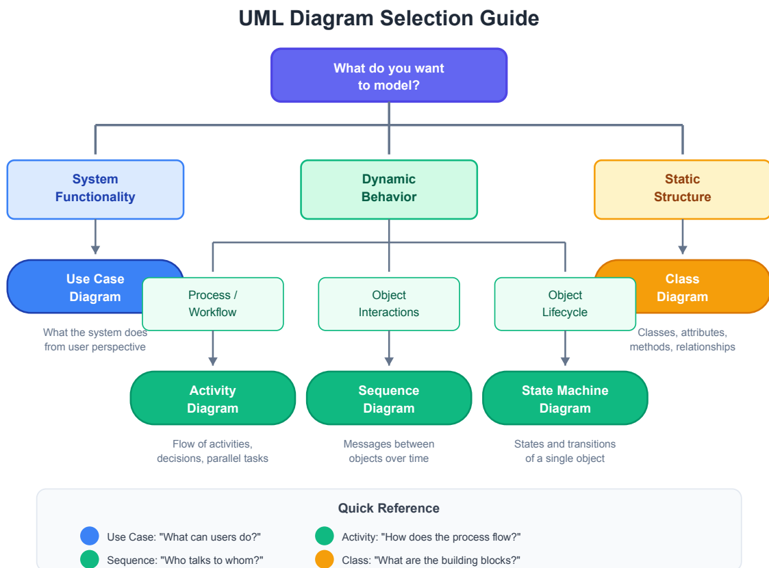
Figure 3.14: Diagram Selection Guide
