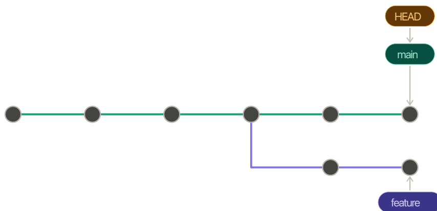
Figure 7.2: Git HEAD pointing to the current branch
