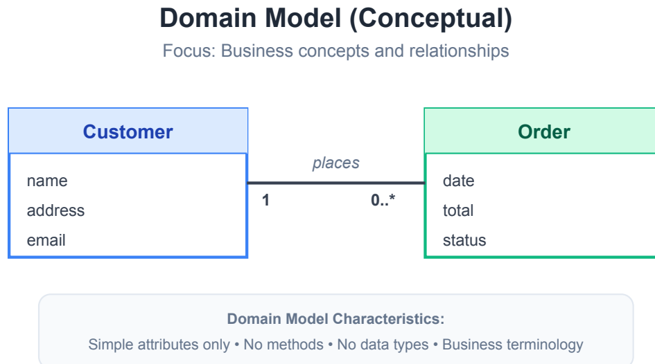
Figure 3.12: Domain Model Example
