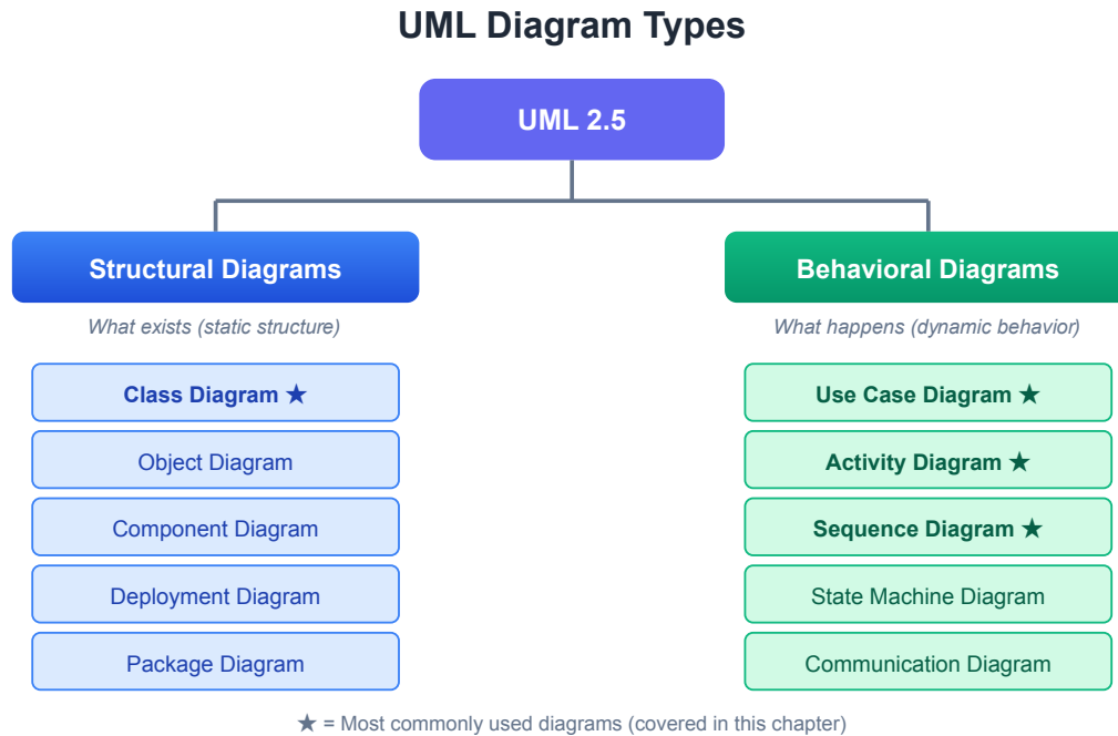
Figure 3.1: UML Diagram Types
