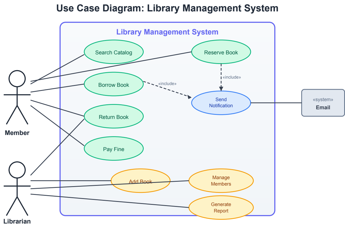
Figure 3.3: Use Case Diagram Example
