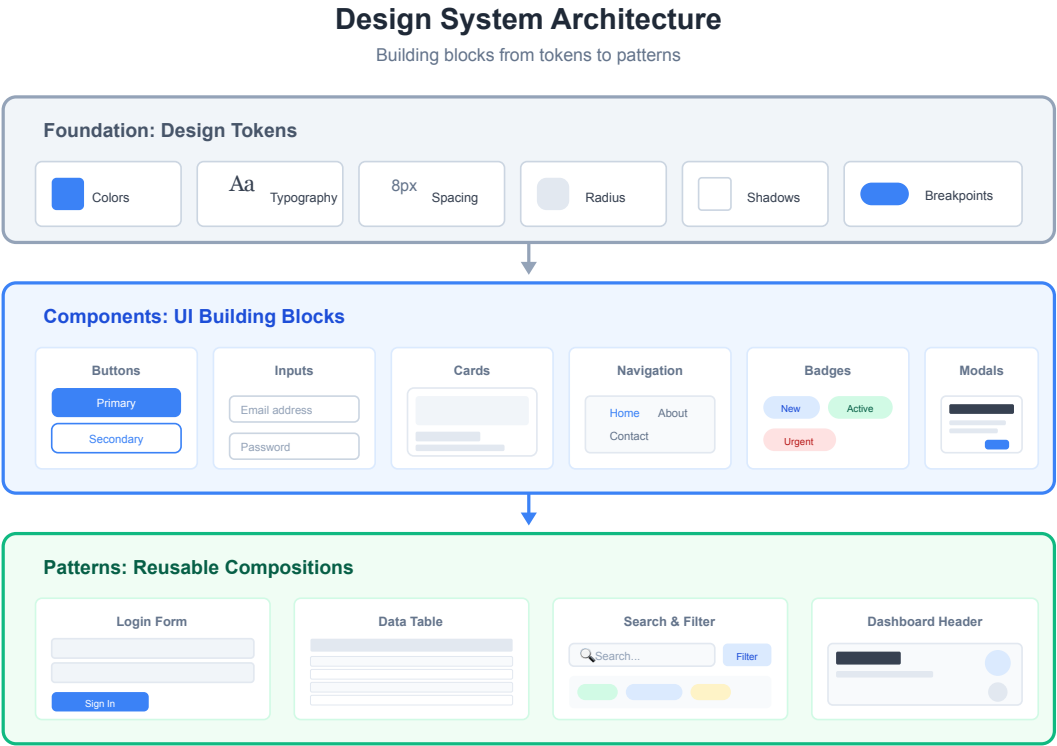
Figure 5.8: Design System Architecture
