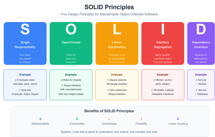
Figure 4.12: SOLID Principles
