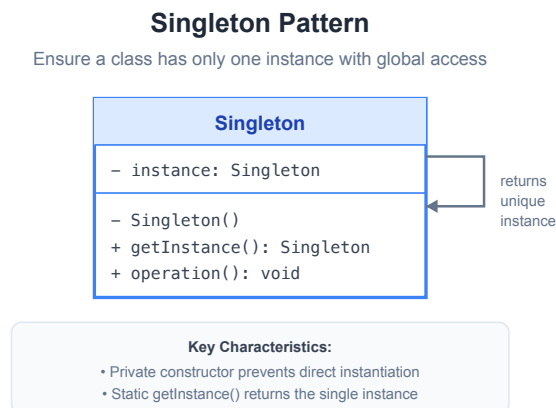
Figure 4.14: Singleton Pattern
