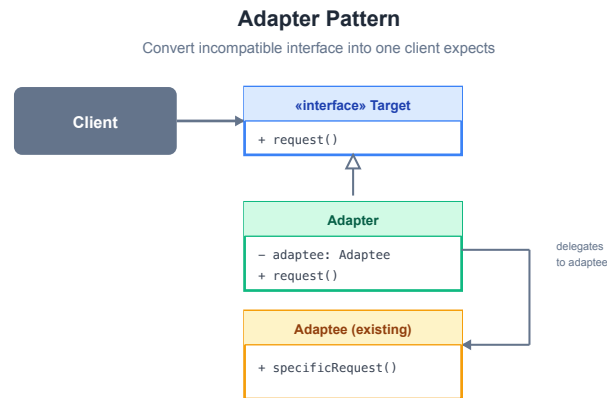
Figure 4.18: Adapter Pattern
