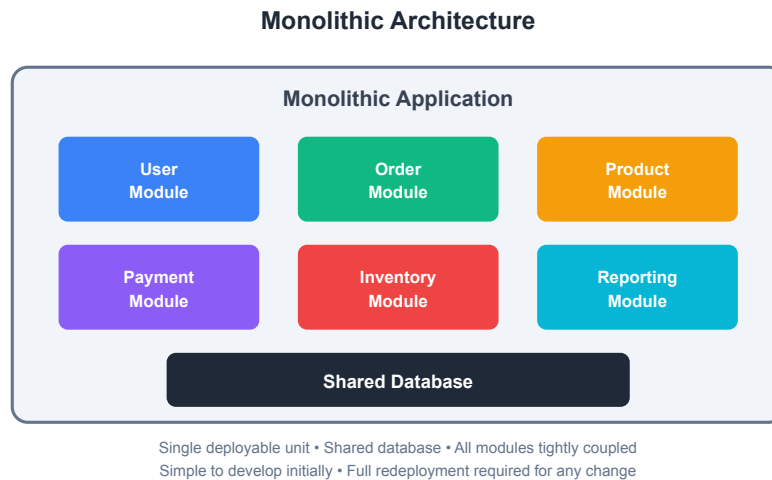
Figure 4.9: Monolithic Architecture
