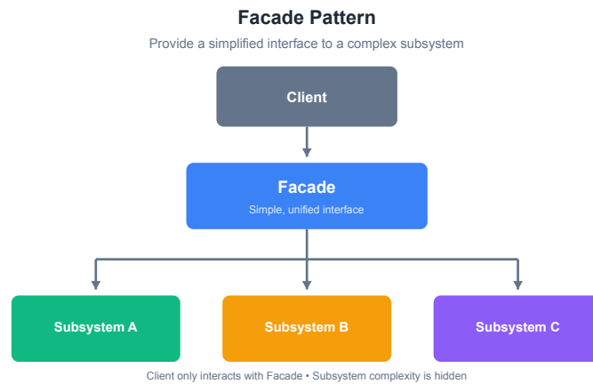
Figure 4.20: Facade Pattern
