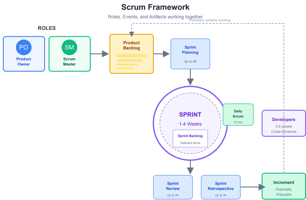
Figure 6.2: Scrum Framework
