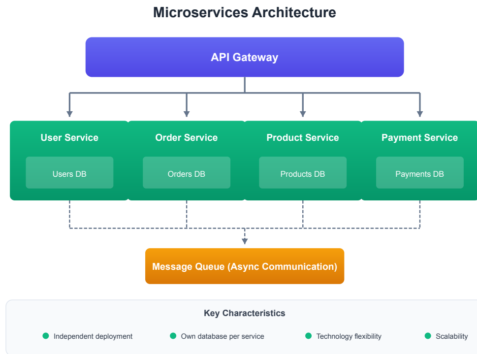
Figure 4.6: Microservices Architecture
