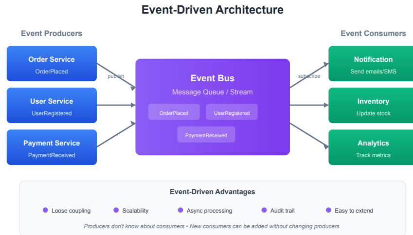
Figure 4.7: Event-Driven Architecture
