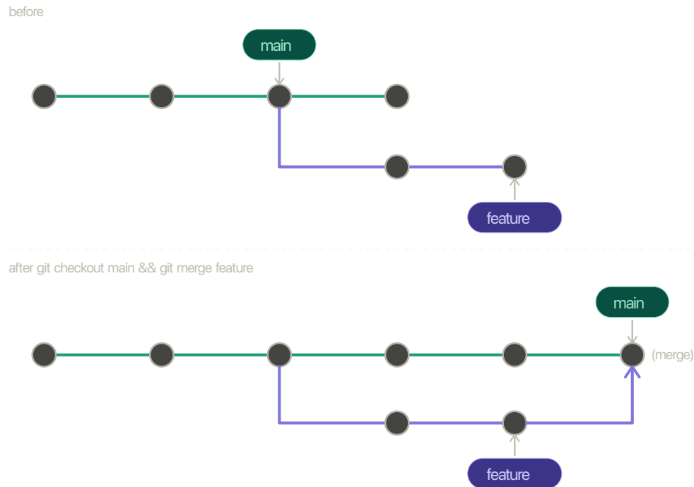
Figure 7.5: Three-way Git merge creating a merge commit
