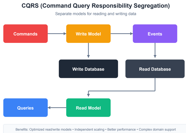
Figure 4.8: CQRS (Command Query Responsibility Segregation)
