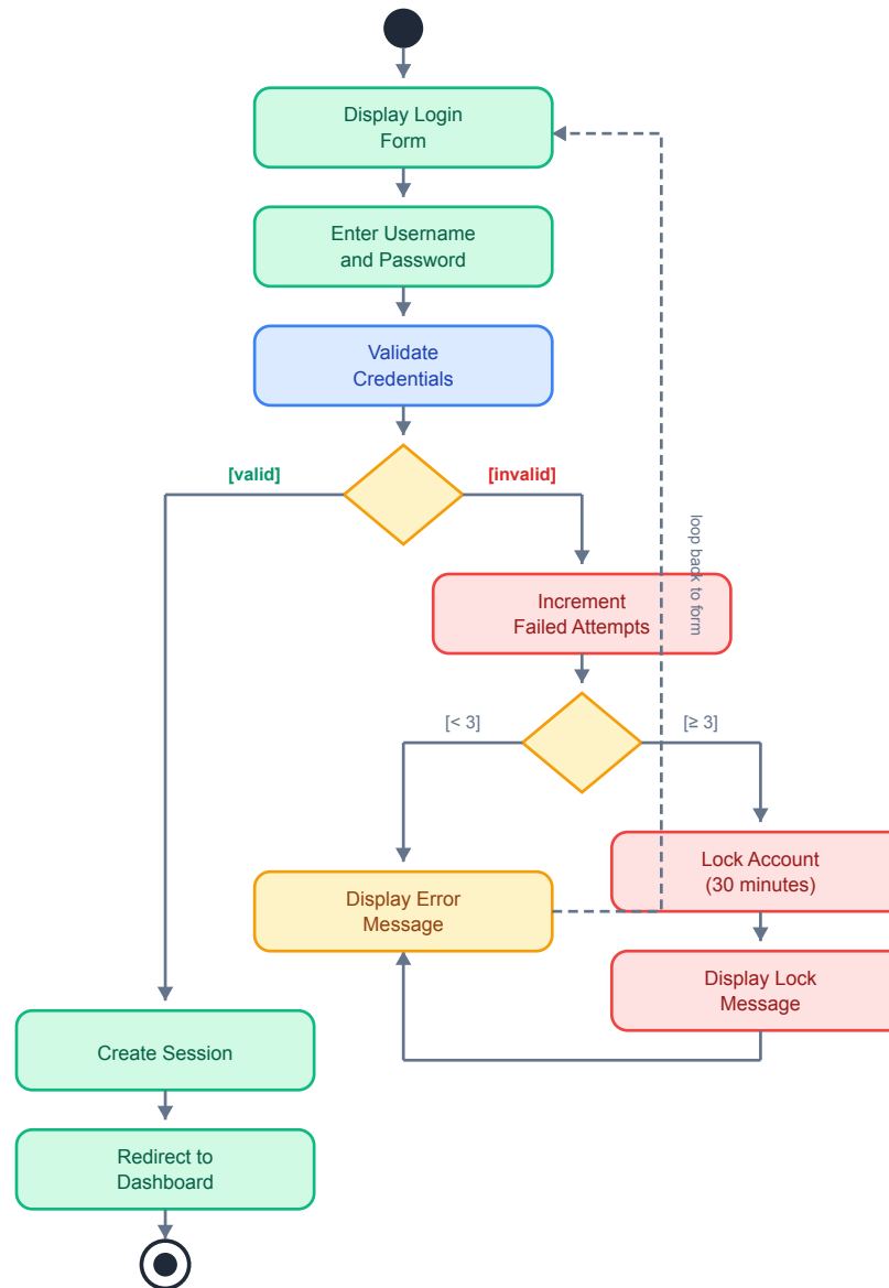
Figure 3.6: Login activity diagram with validation, retry, session creation, and dashboard redirection
