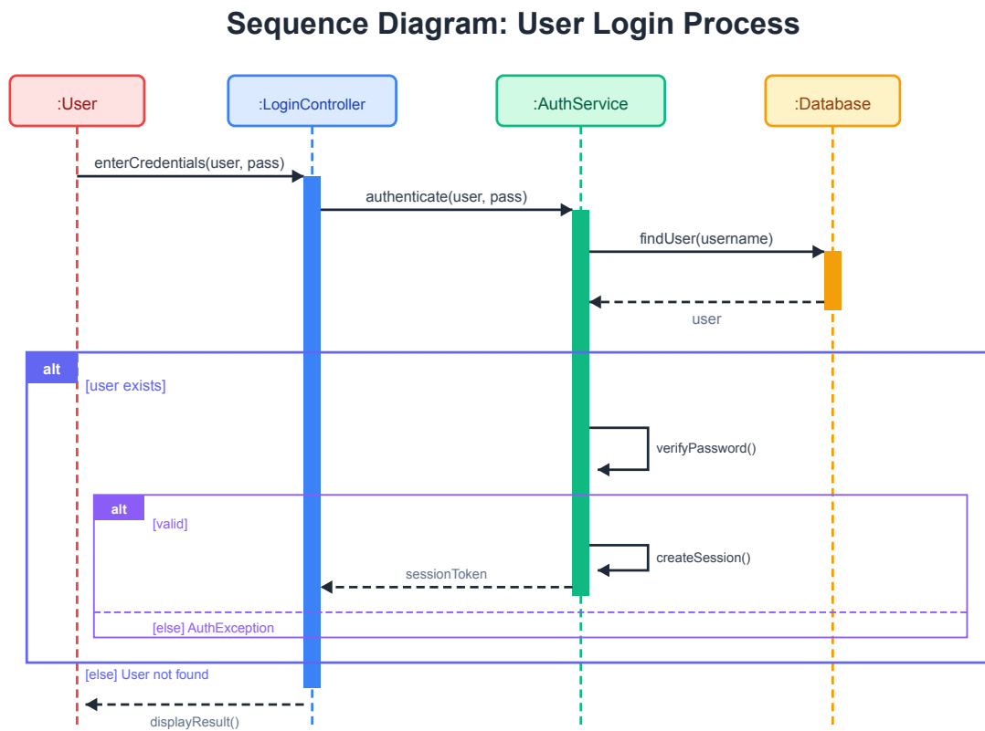
Figure 3.8: Sequence Diagram Example
