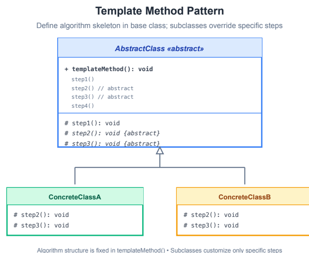
Figure 4.23: Template Method Pattern
