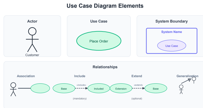
Figure 3.2: UML notation for actors, use cases, system boundaries, and associations
