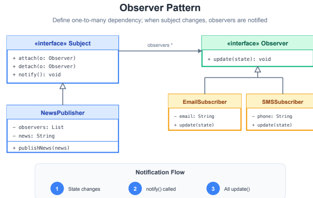
Figure 4.22: Observer Pattern
