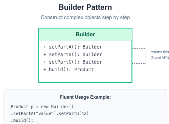
Figure 4.17: Builder Pattern
