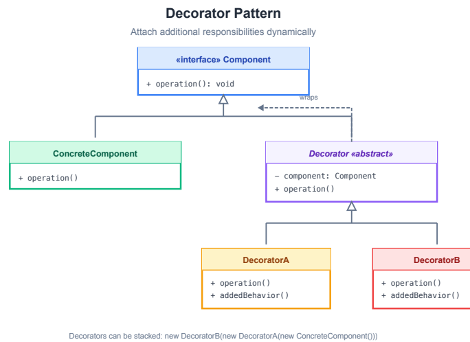
Figure 4.19: Decorator Pattern
