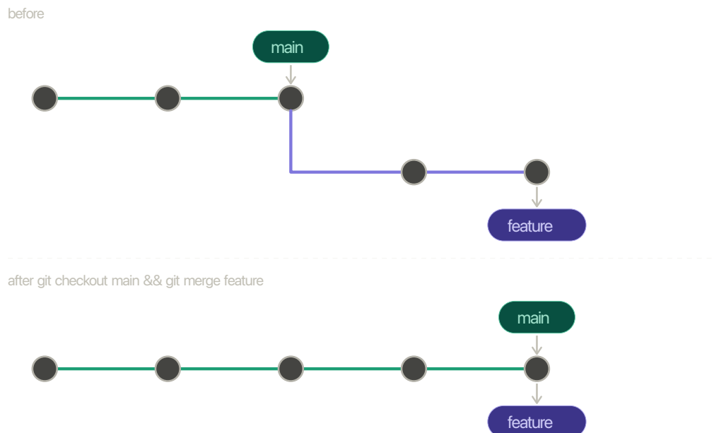
Figure 7.4: Fast-forward merge before and after
