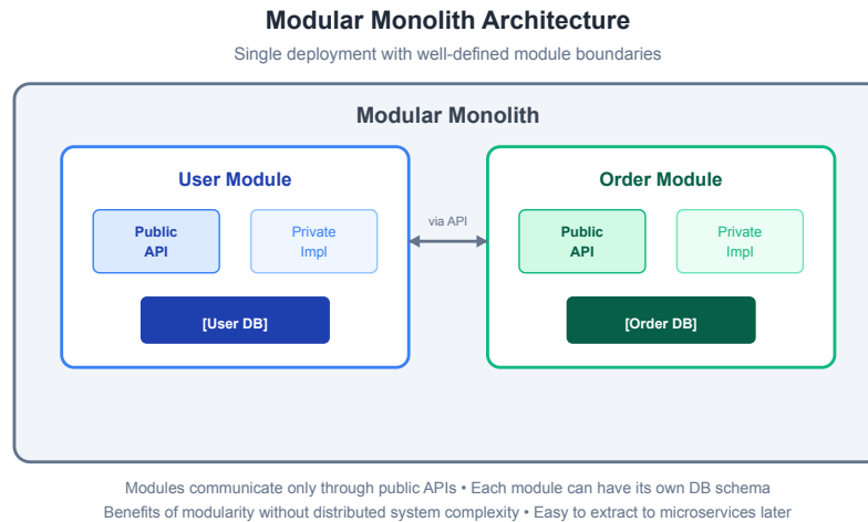
Figure 4.10: Modular Monolith Architecture
