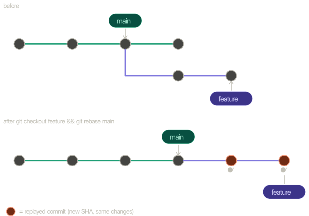
Figure 7.6: Git history before and after rebasing a feature branch
