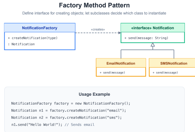
Figure 4.15: Factory Method Pattern
