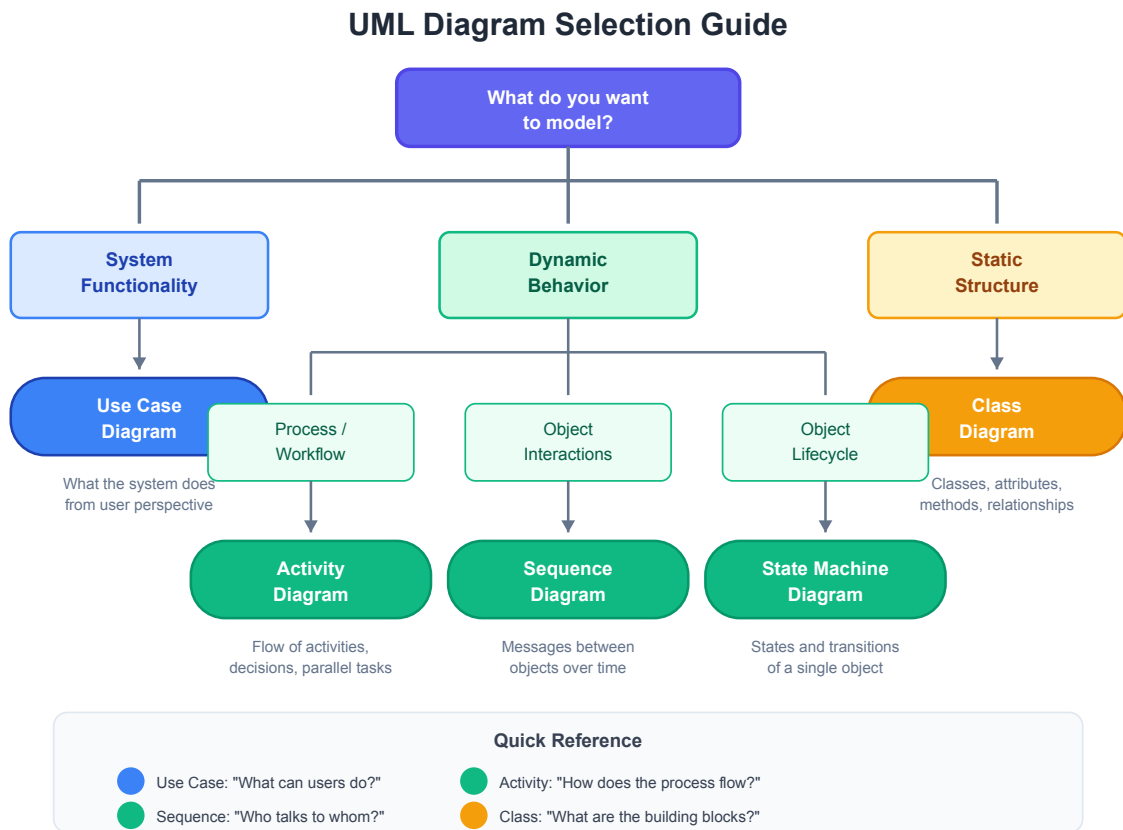
Figure 3.13: Diagram Selection Guide
