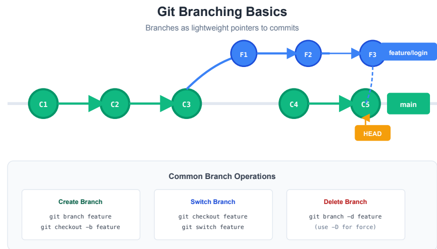
Figure 7.1: Git branching basics - branches as pointers
