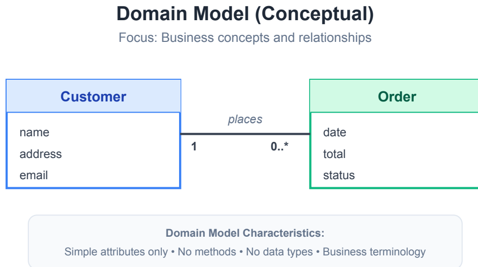
Figure 3.11: Domain Model Example
