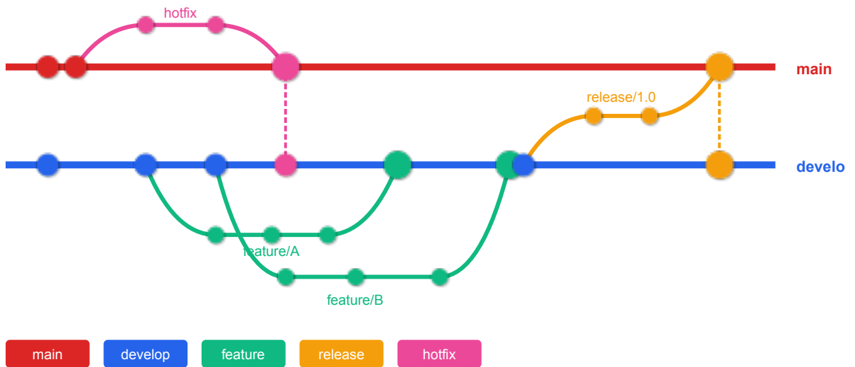
Figure 1.7: Gitflow
