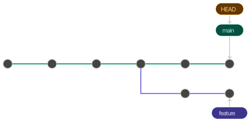
Figure 7.2: Git HEAD pointing to the current branch
