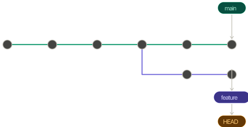
Figure 7.3: Git HEAD after checking out a feature branch
