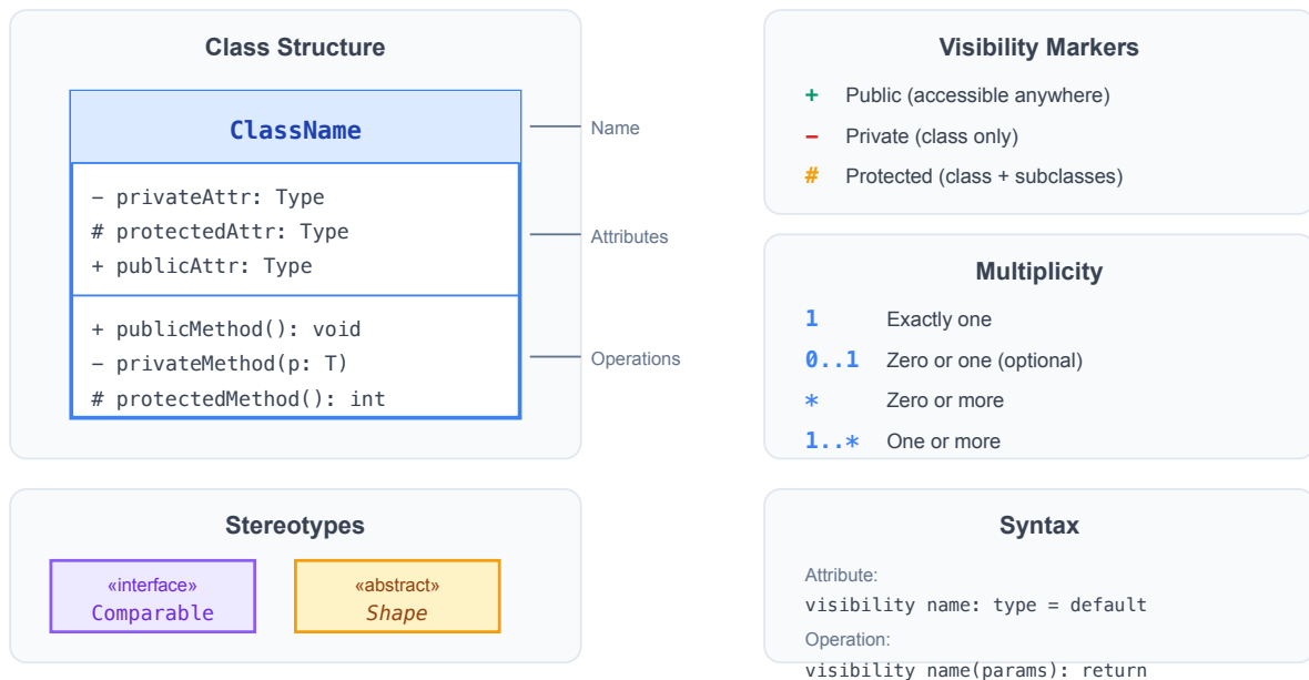
Figure 3.8: Class Notation
