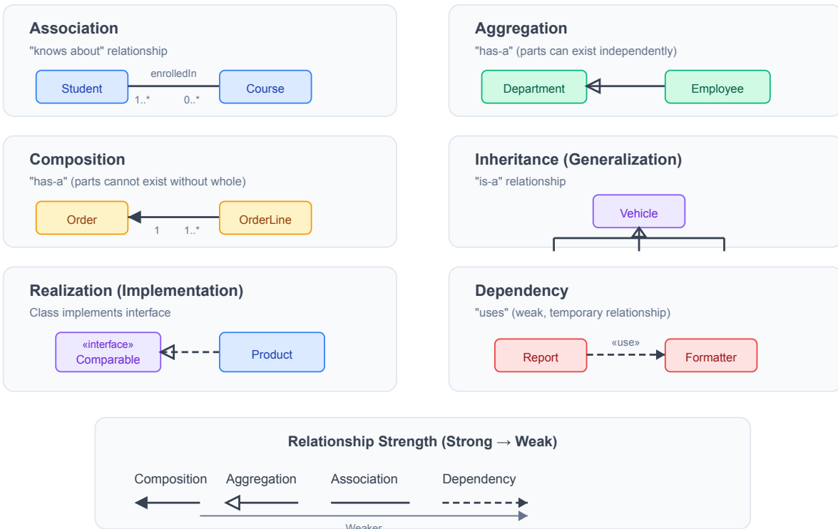
Figure 3.9: Class Relationships
