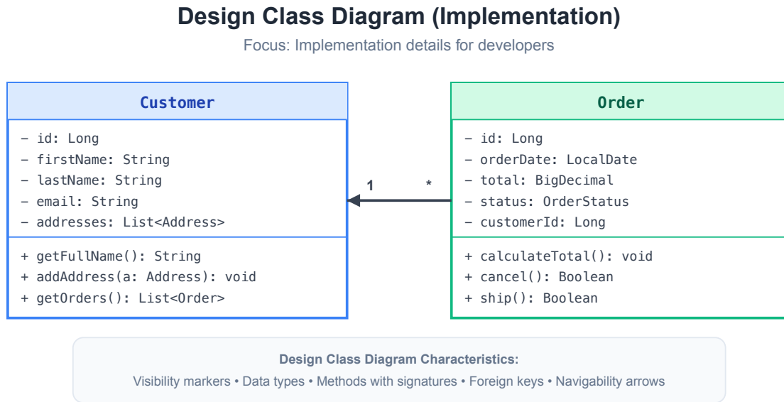
Figure 3.12: Design Class Diagram Example
