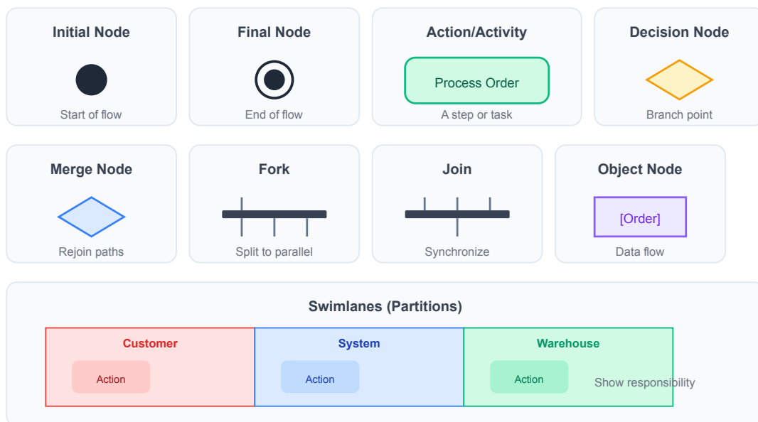
Figure 3.4: Activity Diagram Elements
