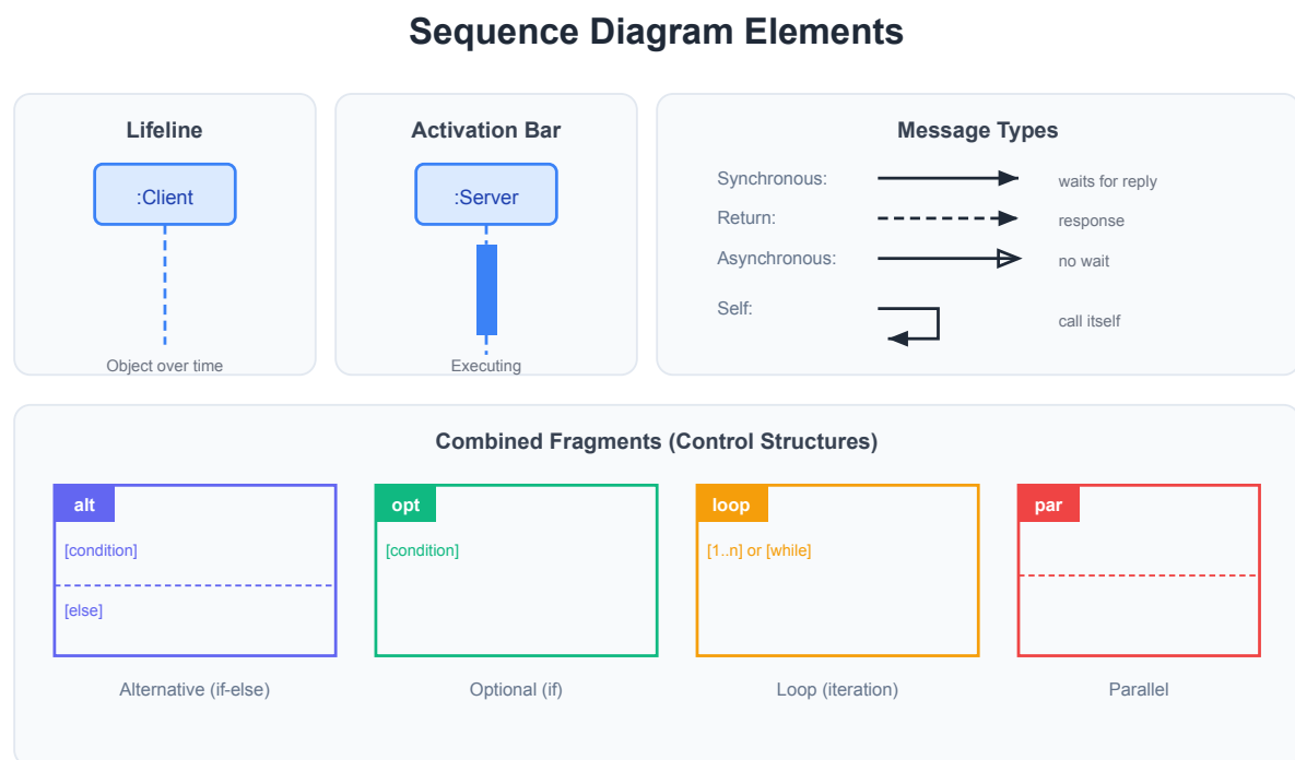
Figure 3.6: Sequence Diagram Elements
