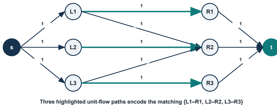
Figure 9.4: A source connects to three left vertices, compatibility edges connect the bipartition, and three highlighted unit-flow paths reach the sink through distinct right vertices.
