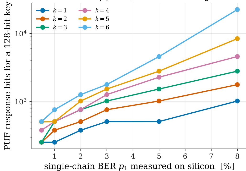
(b) Silicon-transfer nomogram measure p_1 once, read off the budget
