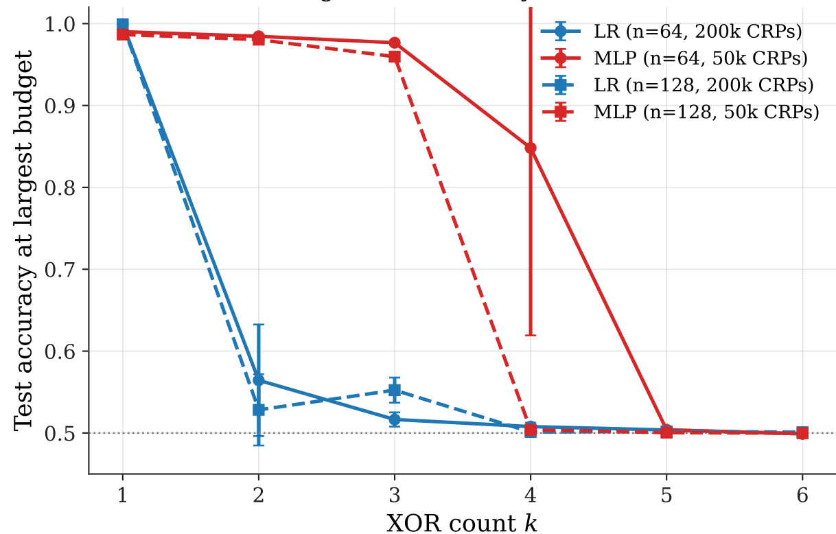
Modeling-attack accuracy vs XOR count
