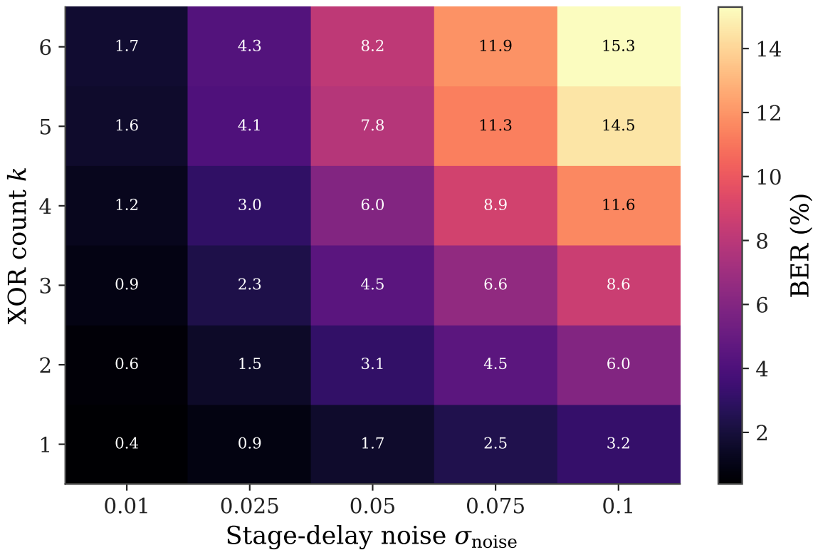
Intra-device BER (%) over (\sigma, k) , n = 64
