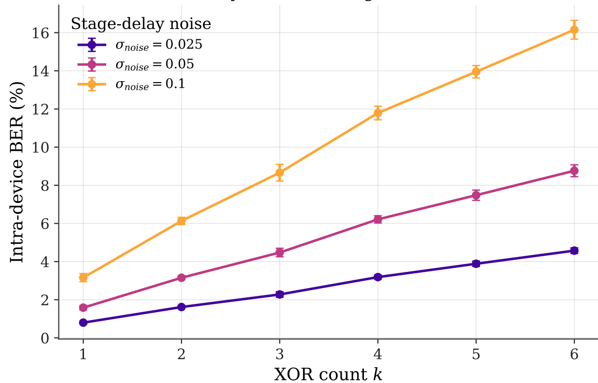
Reliability cost of XORing (64-bit chains)
