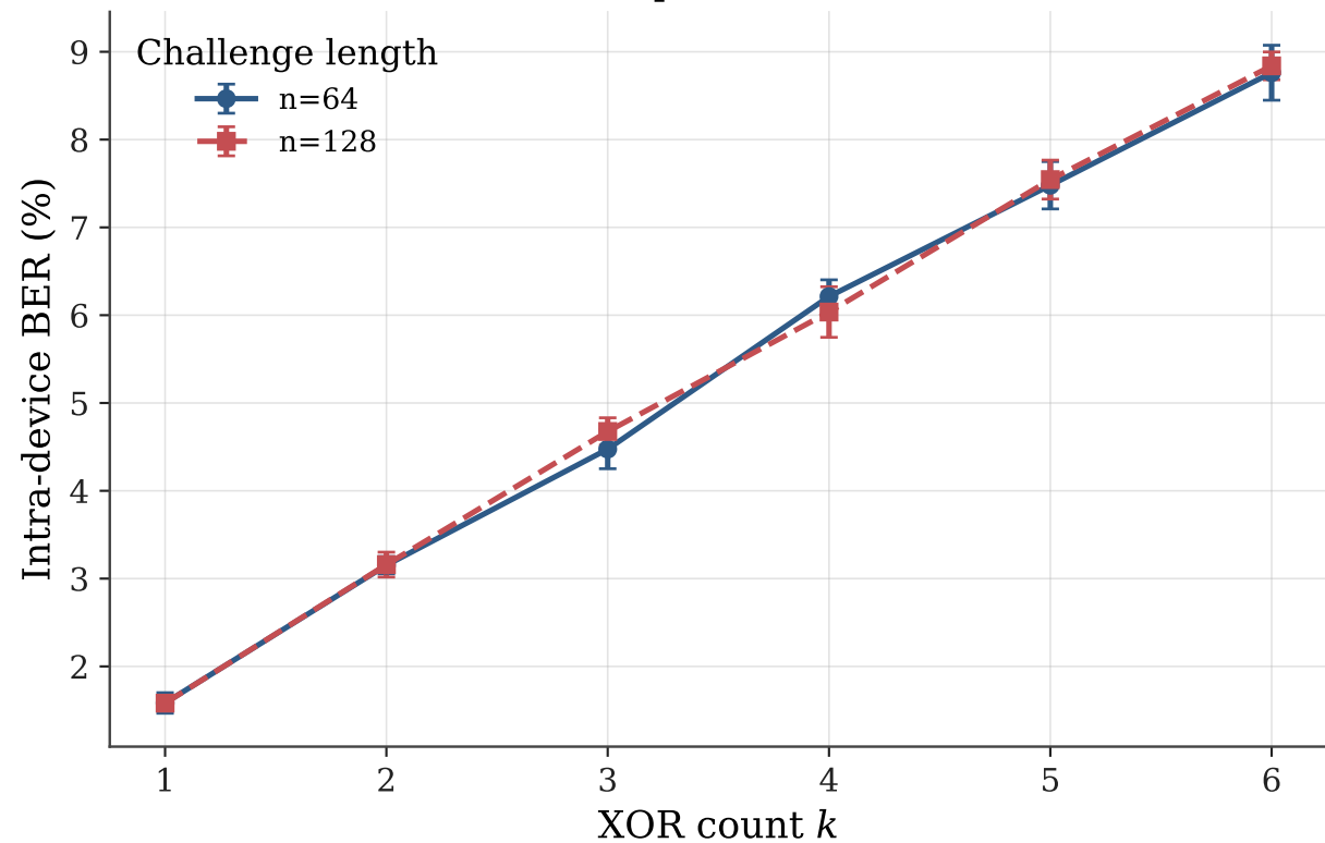
BER vs k is independent of n ( \sigma = 0.05 )
