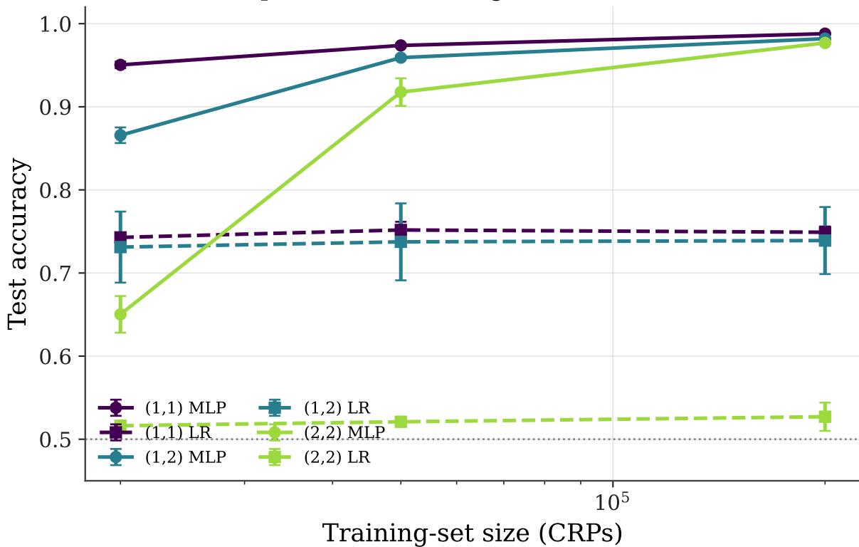
Interpose-PUF modeling resistance ( n = 64 )
