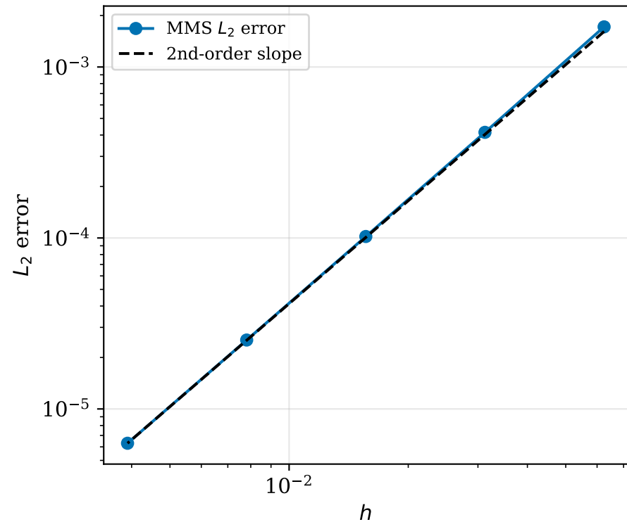
Poisson operator (order \approx 2.01 )
