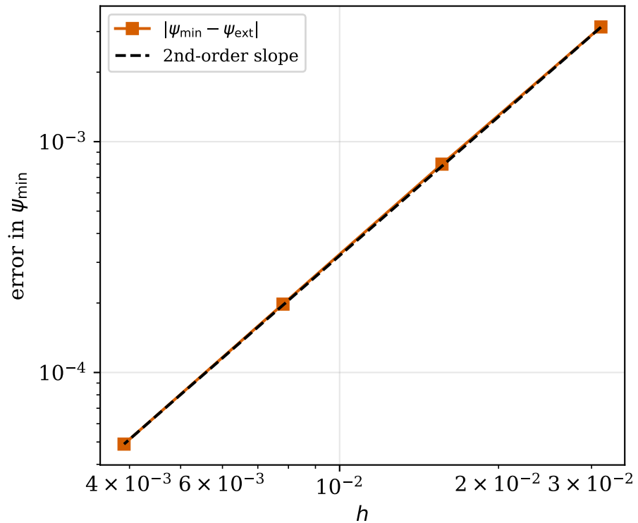
Primary vortex (order \approx 2.01 )
